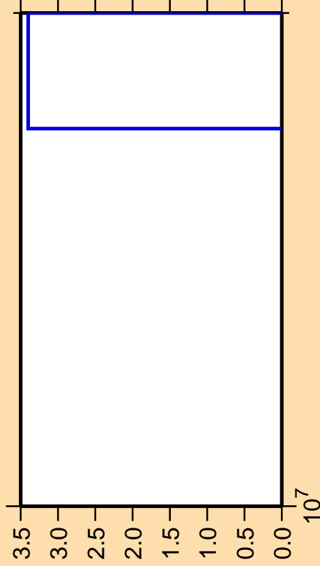
\Delta\sigma/\sigma vs. E for ^{130}\text{Sn}(n,\text{nd})
