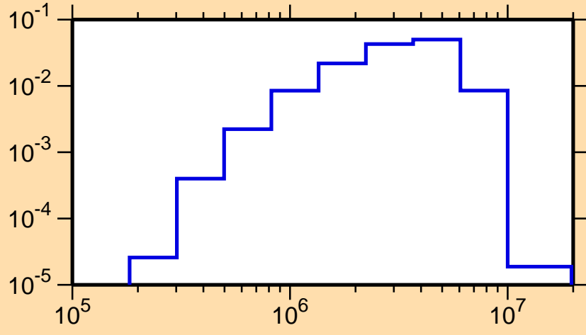
\sigma vs. E for ^{131}\text{Sn}(n,n_2)
