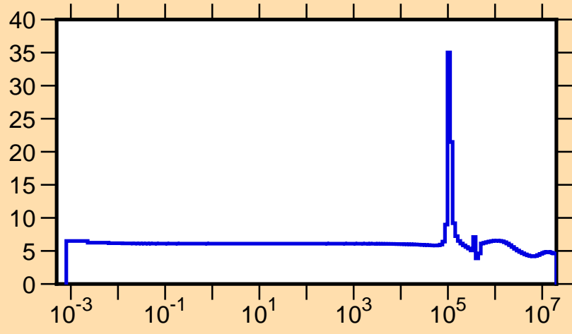
\sigma vs. E for ^{132}\text{Sn}(n,\text{tot.})
