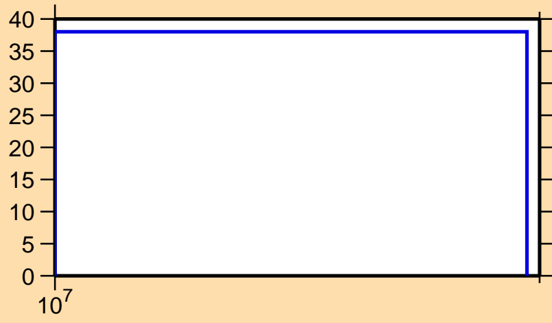
\Delta\sigma/\sigma vs. E for ^{132}\text{Sn}(n,el.)
