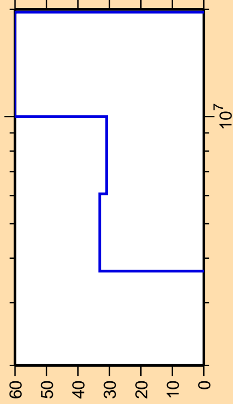
\Delta\sigma/\sigma vs. E for ^{132}\text{Sn}(n,n_3)
