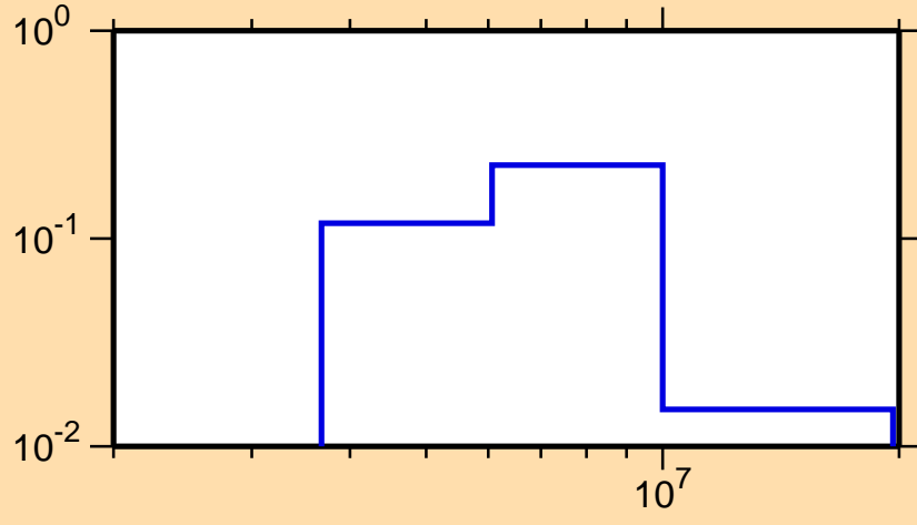
\sigma vs. E for ^{132}\text{Sn}(n,n_3)
