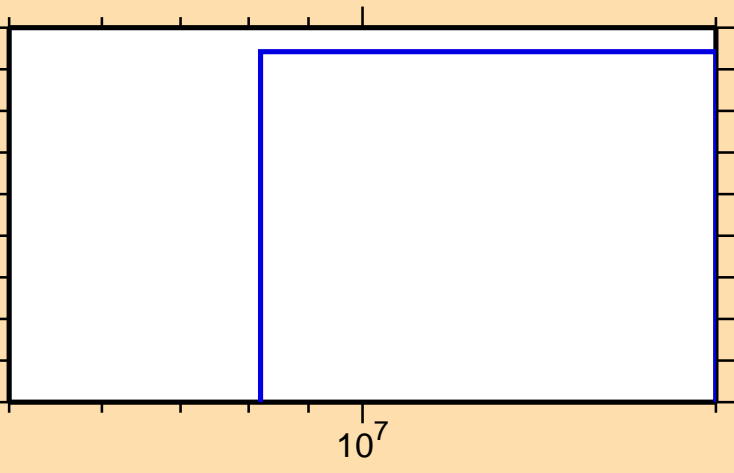
\sigma vs. E for ^{132}\text{Sn}(n,n\alpha)
