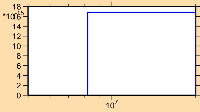
\sigma vs. E for ^{132}\text{Sn}(n,n\alpha)
