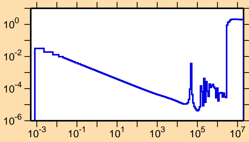
\sigma vs. E for ^{133}\text{Sn}(n,\text{nonel.})
