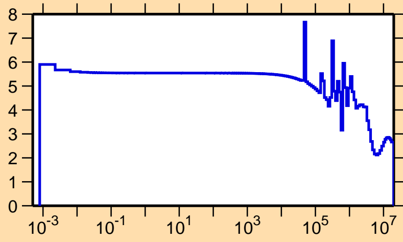
\sigma vs. E for ^{133}\text{Sn}(n,\text{el.})
