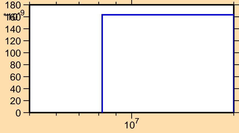
\sigma vs. E for ^{133}\text{Sn}(n,t)
