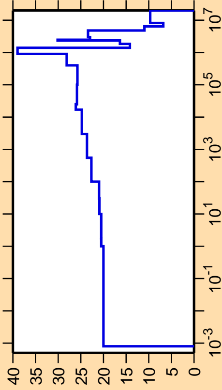
\Delta\sigma/\sigma vs. E for ^{133}\text{Sn}(n,\text{el.})
