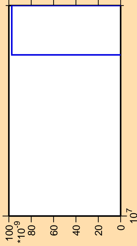
\Delta\sigma/\sigma vs. E for ^{134}\text{Sn} (mt 11)
