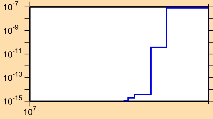
\sigma vs. E for ^{134}\text{Sn}(n,d)
