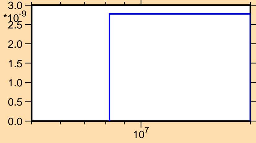
\sigma vs. E for ^{134}\text{Sn}(n,\alpha)
