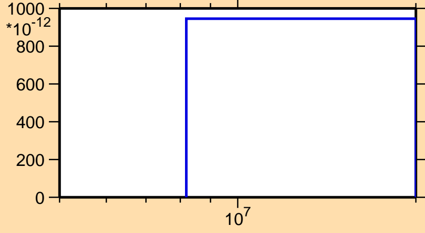
\sigma vs. E for ^{134}\text{Sn}(n,p)
