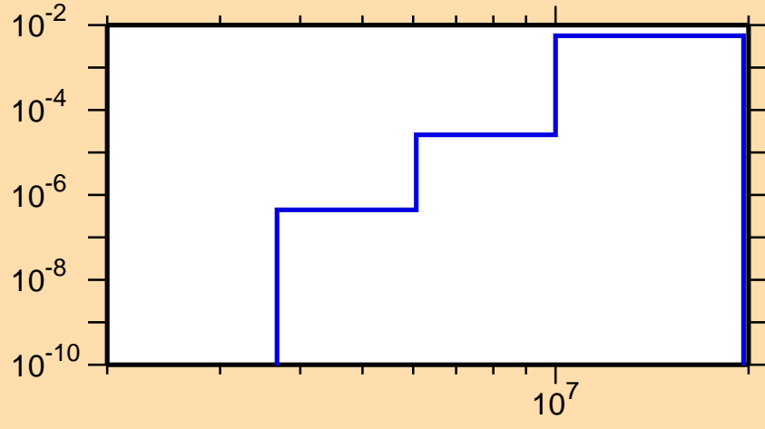
\sigma vs. E for ^{76}\text{Sr}(n,d)
