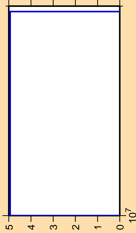
\Delta\sigma/\sigma vs. E for ^{76}\text{Sr} (mt 34)
