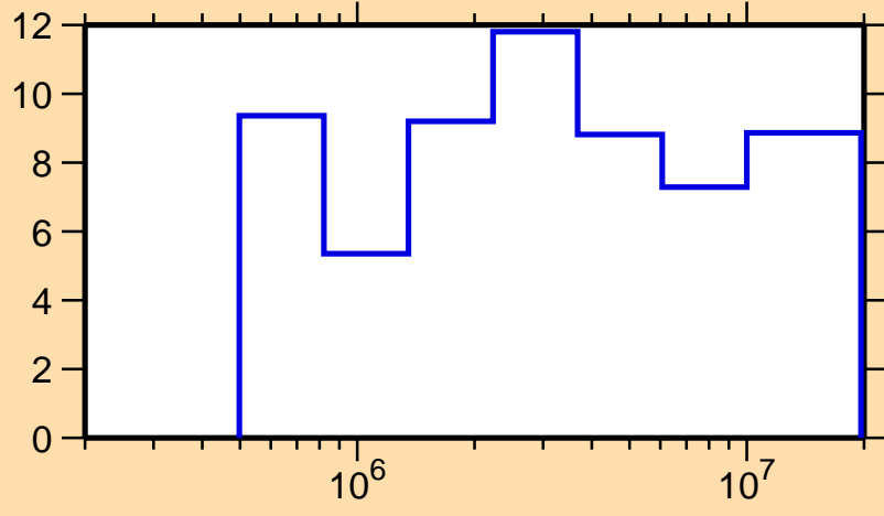
\Delta\sigma/\sigma vs. E for ^{76}\text{Sr}(n,n\text{onel.})
