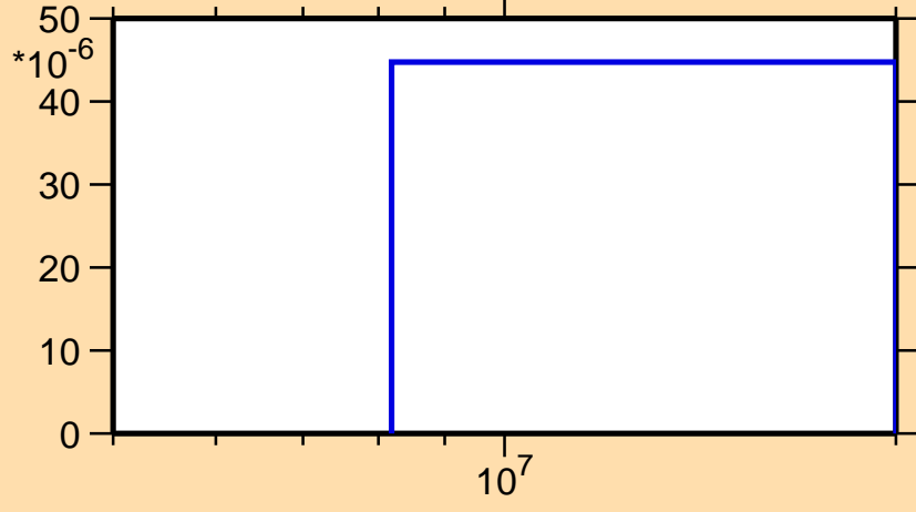
\sigma vs. E for ^{76}\text{Sr}(n,t)
