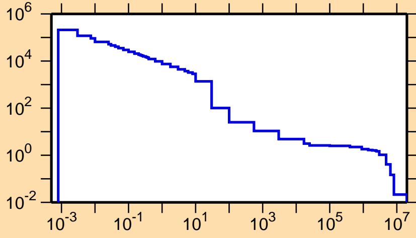
\sigma vs. E for ^{76}\text{Sr}(n,p)
