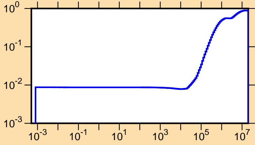
\mu vs. E for ^{77}\text{Sr}(\text{mt251})
