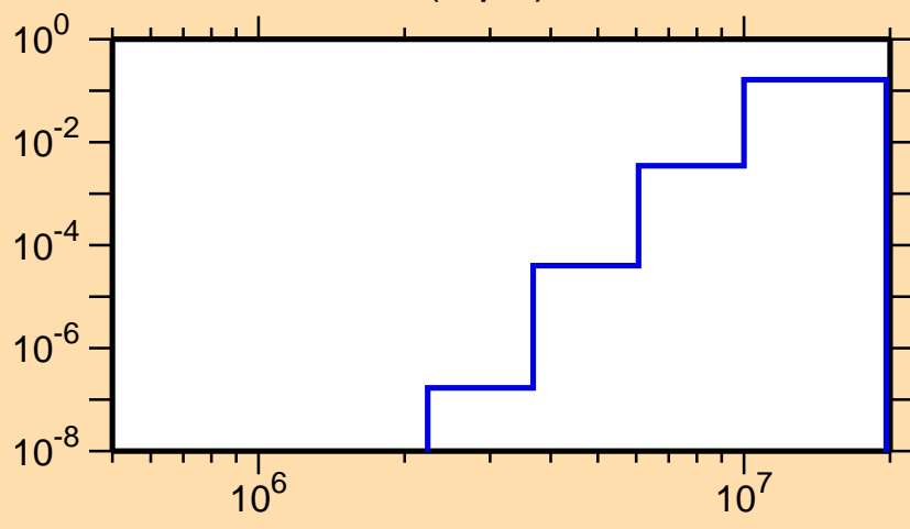
\sigma vs. E for ^{77}\text{Sr}(n,p\alpha)
