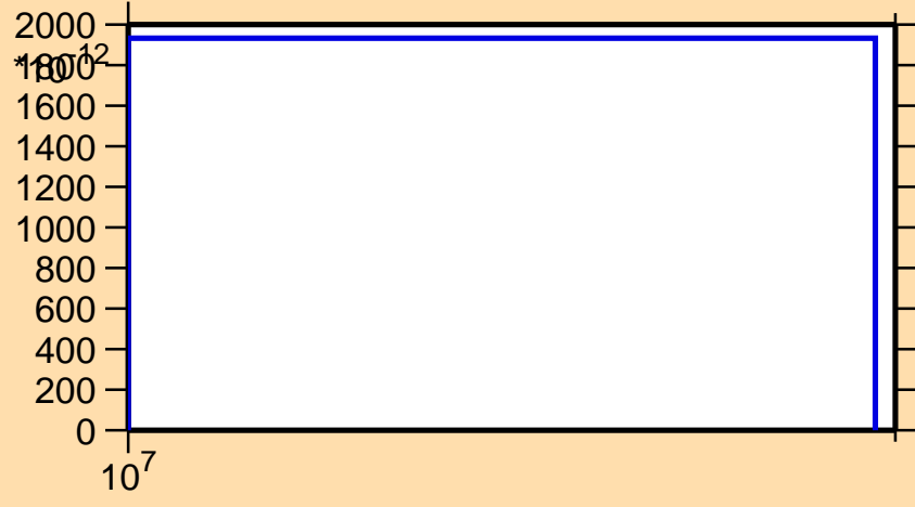
\sigma vs. E for ^{77}\text{Sr} (mt 45)
