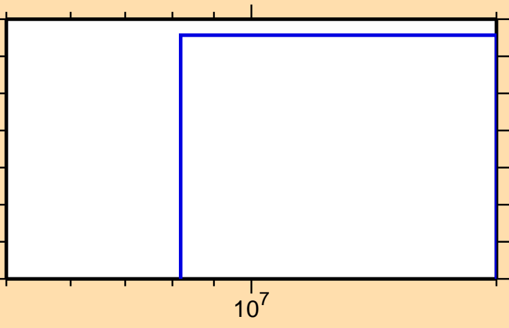
\sigma vs. E for ^{77}\text{Sr}(n,\text{pt})
