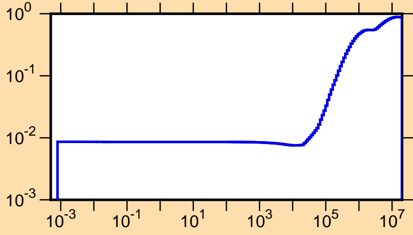
\mu vs. E for ^{78}\text{Sr}(\text{mt251})
