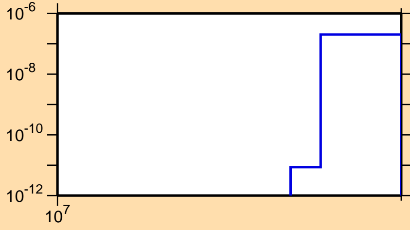
\sigma vs. E for ^{78}\text{Sr}(n,\text{pt})
