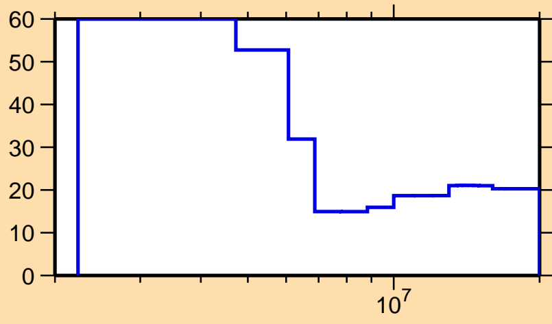
\Delta\sigma/\sigma vs. E for ^{78}\text{Sr}(n,n\text{cont.})
