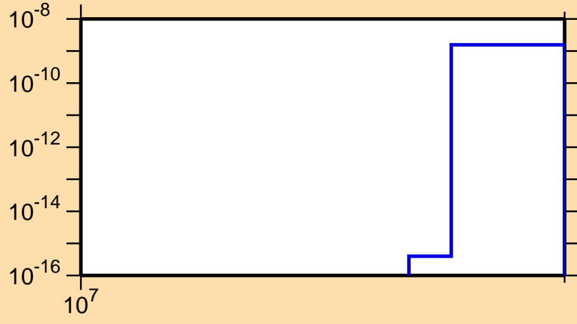
\sigma vs. E for ^{78}\text{Sr}(n,\text{nd})
