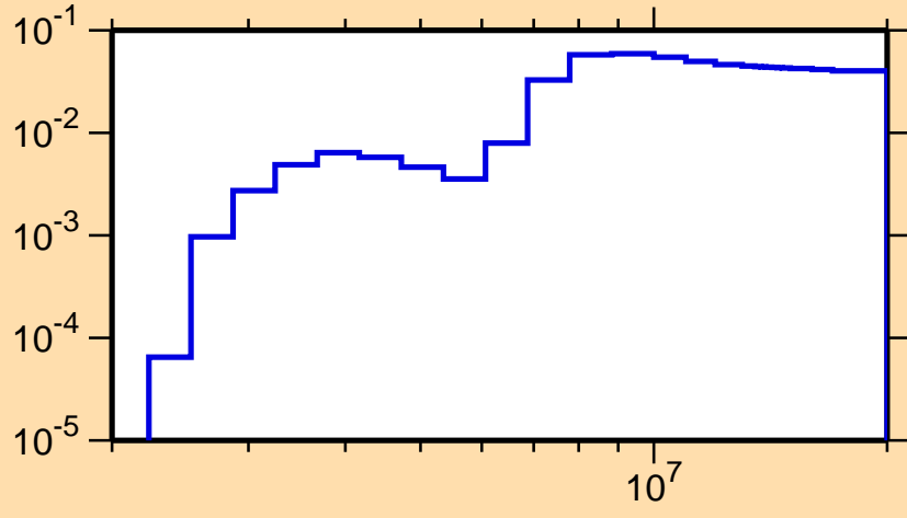
\sigma vs. E for ^{78}\text{Sr}(n,n\text{cont.})
