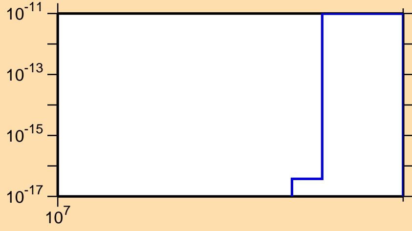
\sigma vs. E for ^{78}\text{Sr} (mt 34)
