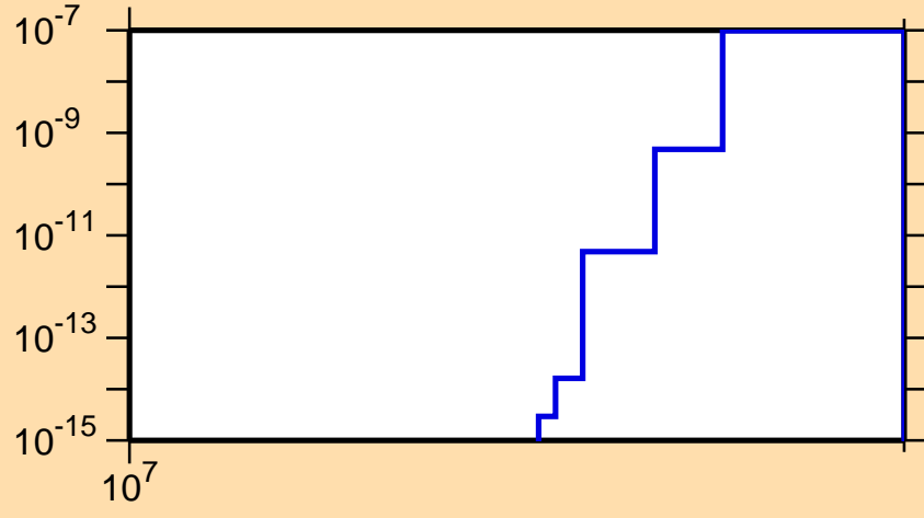
\sigma vs. E for ^{78}\text{Sr} (mt 45)
