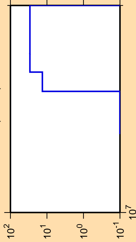
\Delta\sigma/\sigma vs. E for ^{78}\text{Sr} (mt 45)
