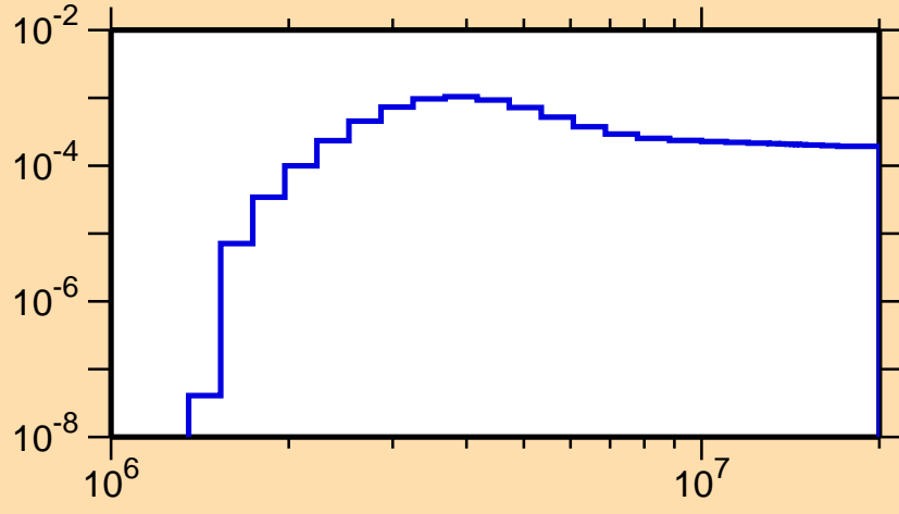
\sigma vs. E for ^{78}\text{Sr}(n,n_4)
