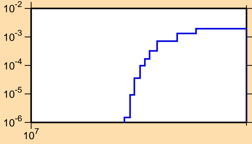
\sigma vs. E for ^{78}\text{Sr}(n,2n)
