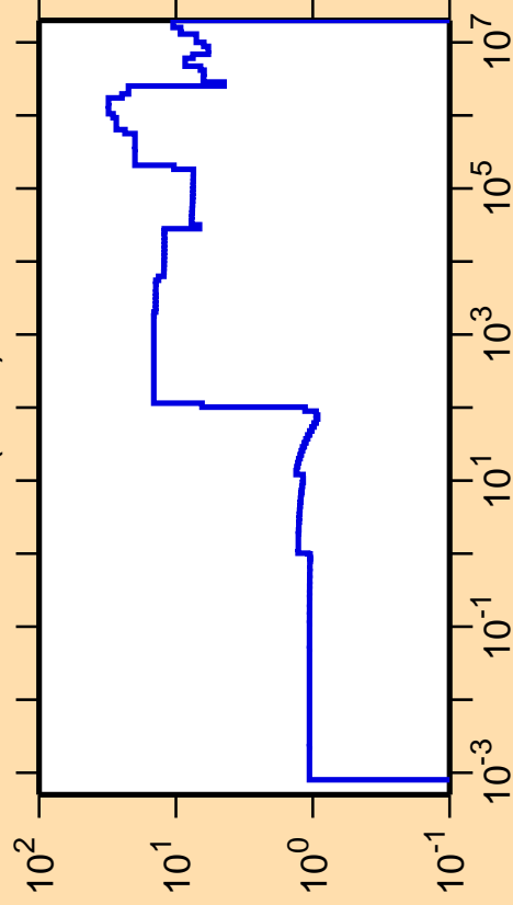
\Delta\sigma/\sigma vs. E for ^{78}\text{Sr}(n,\text{el.})
