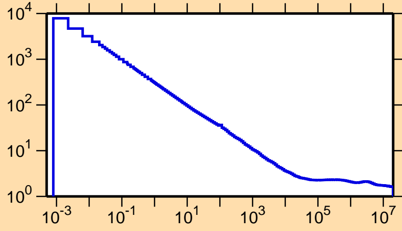
\sigma vs. E for ^{78}\text{Sr}(n,\text{nonel.})
