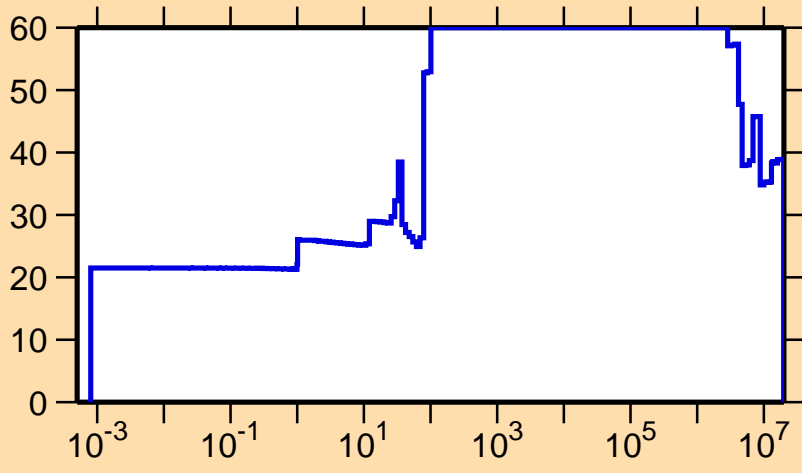
\Delta\sigma/\sigma vs. E for ^{78}\text{Sr}(n,\gamma)
