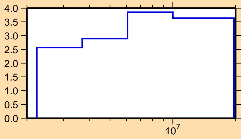
\Delta\sigma/\sigma vs. E for ^{78}\text{Sr}(n,n\text{onel.})
