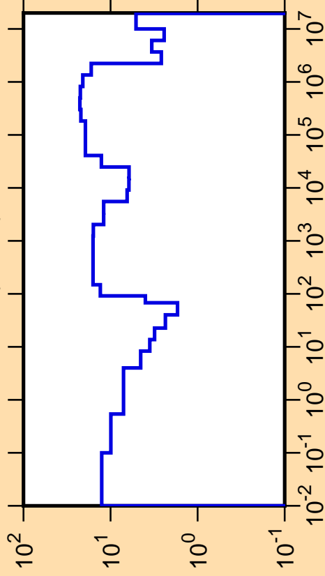
\Delta\sigma/\sigma vs. E for ^{78}\text{Sr}(n,\text{tot.})
