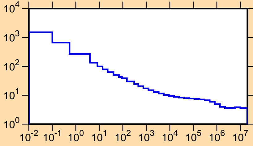
\sigma vs. E for ^{78}\text{Sr}(n,\text{tot.})
