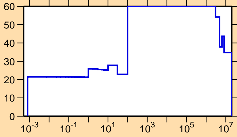
\Delta\sigma/\sigma vs. E for ^{78}\text{Sr}(n,\gamma)
