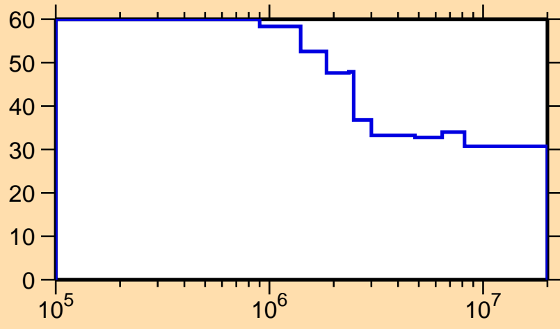
\Delta\sigma/\sigma vs. E for ^{78}\text{Sr}(n,n_1)
