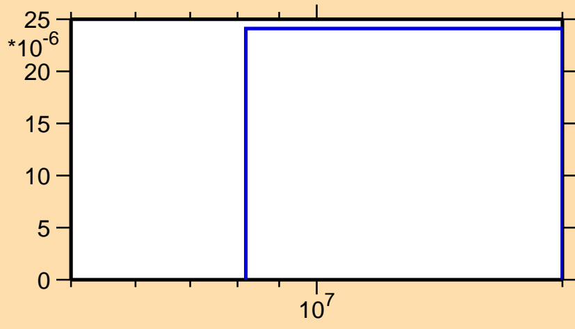
\sigma vs. E for ^{78}\text{Sr}(n,t)
