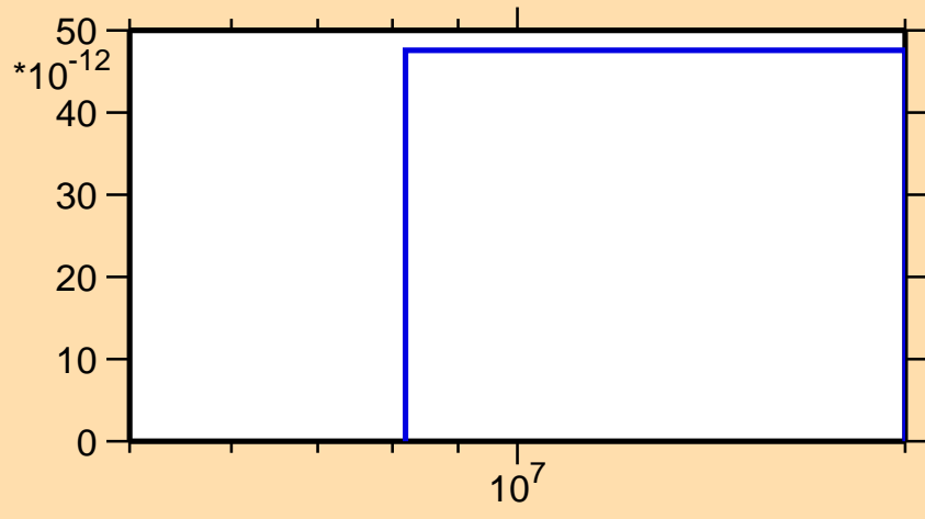
\sigma vs. E for ^{78}\text{Sr}(\text{mt117})
