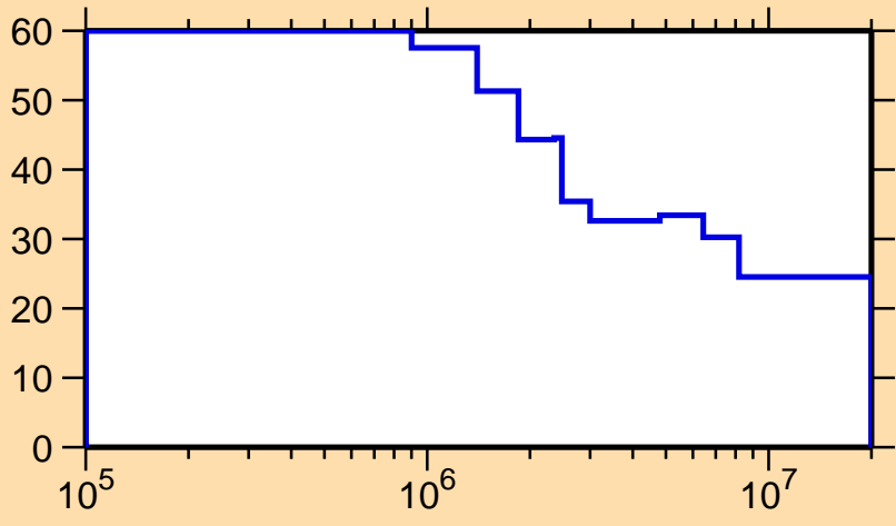
\Delta\sigma/\sigma vs. E for ^{78}\text{Sr}(n,\text{inel.})
