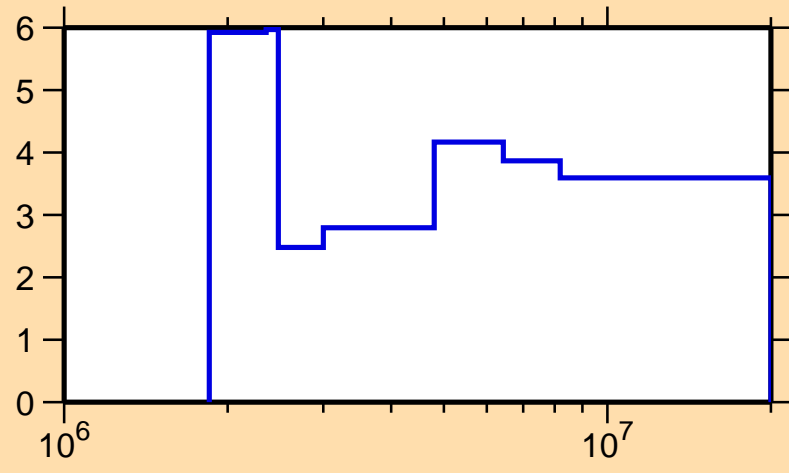
\Delta\sigma/\sigma vs. E for ^{78}\text{Sr}(n,\text{nonel.})
