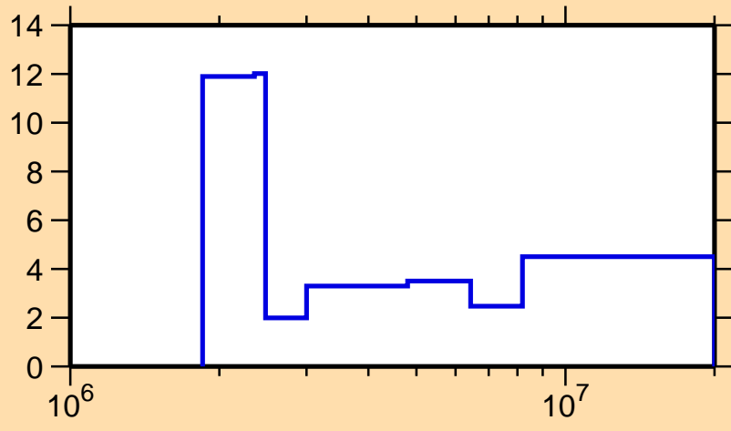
\Delta\sigma/\sigma vs. E for ^{78}\text{Sr}(n,\text{tot.})
