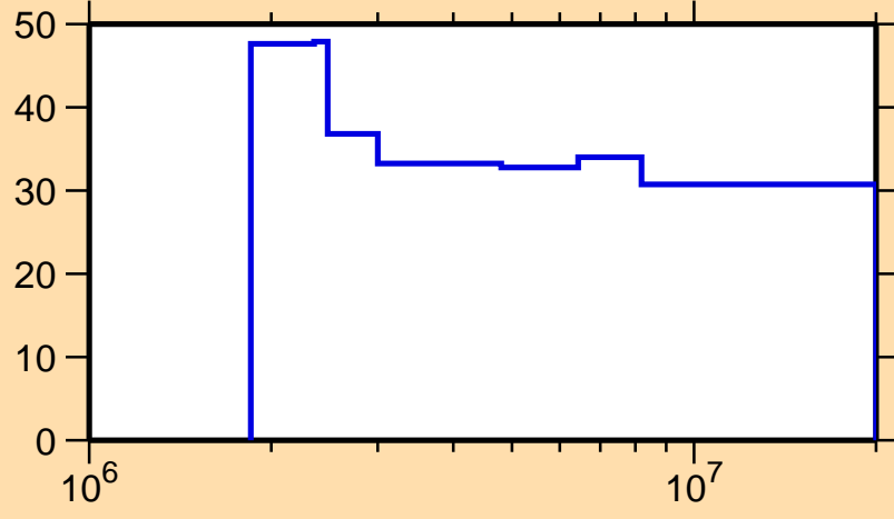
\Delta\sigma/\sigma vs. E for ^{78}\text{Sr}(n,n_1)
