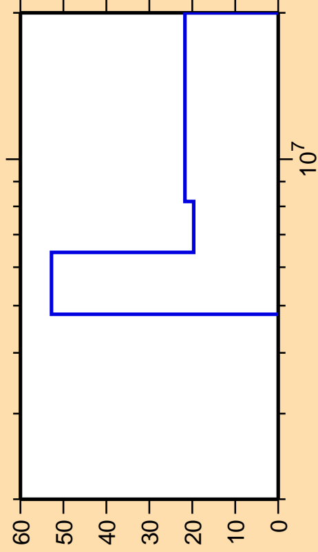
\Delta\sigma/\sigma vs. E for ^{78}\text{Sr}(n,np)
