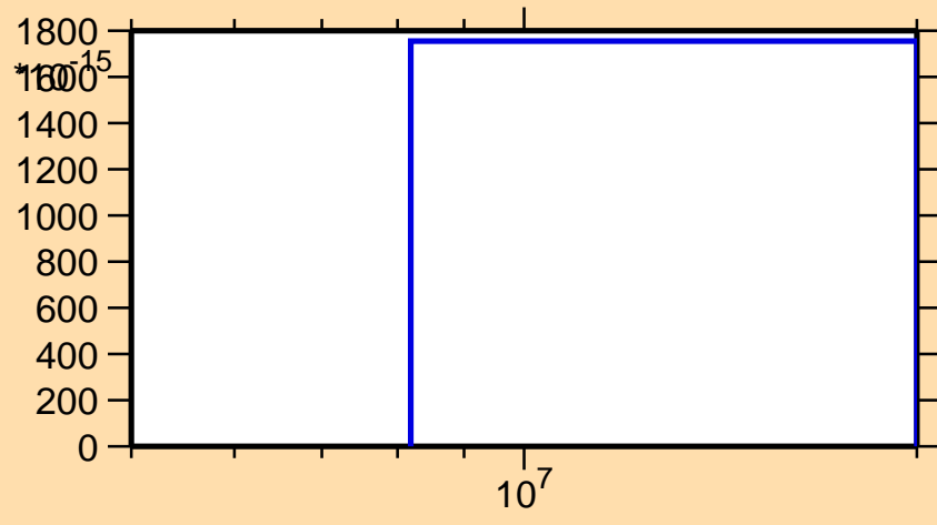
\sigma vs. E for ^{78}\text{Sr}(n,2np)
