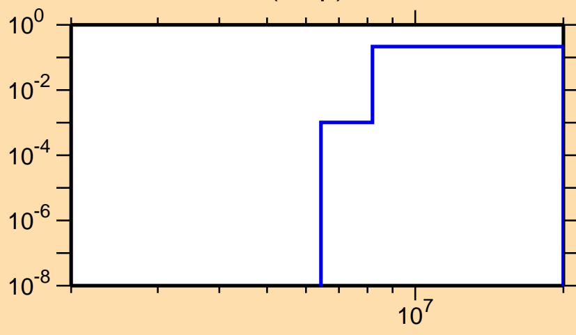
\sigma vs. E for ^{78}\text{Sr}(n,np)
