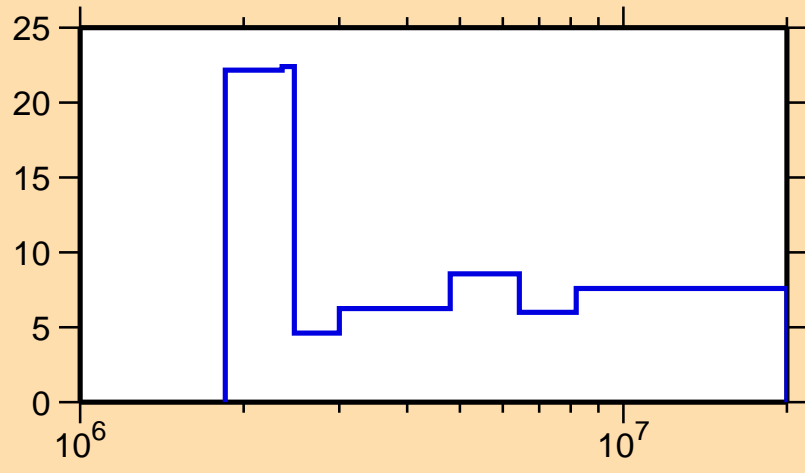
\Delta\sigma/\sigma vs. E for ^{78}\text{Sr}(n,\text{el.})
