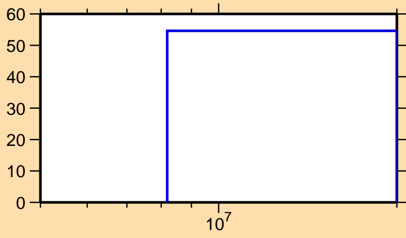
\Delta\sigma/\sigma vs. E for ^{78}\text{Sr}(n,2n)
