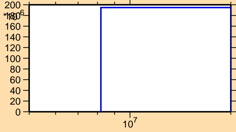
\sigma vs. E for ^{78}\text{Sr}(n,2n)
