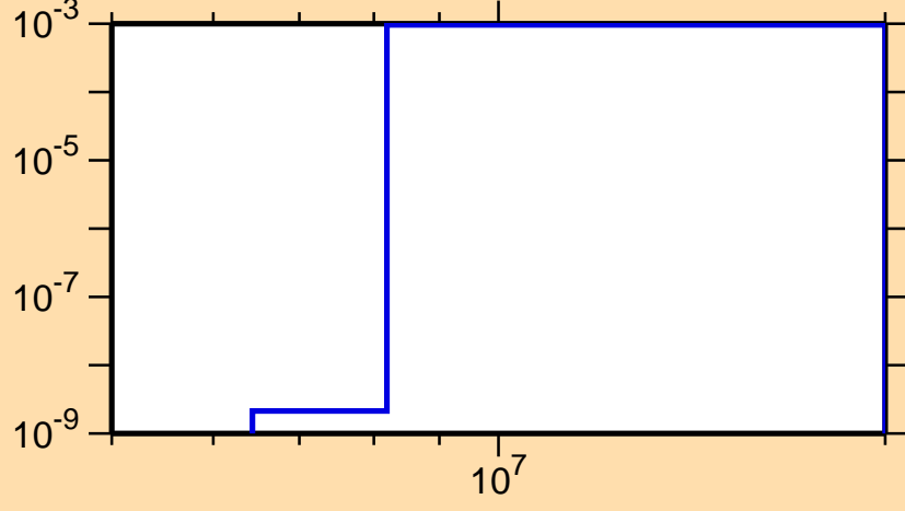
\sigma vs. E for ^{78}\text{Sr}(n,\alpha)
