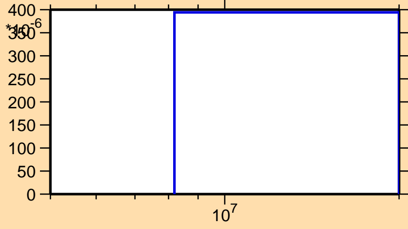
\sigma vs. E for ^{78}\text{Sr}(n,\text{pd})
