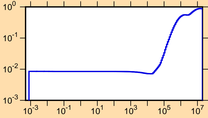
\mu vs. E for ^{79}\text{Sr}(\text{mt251})
