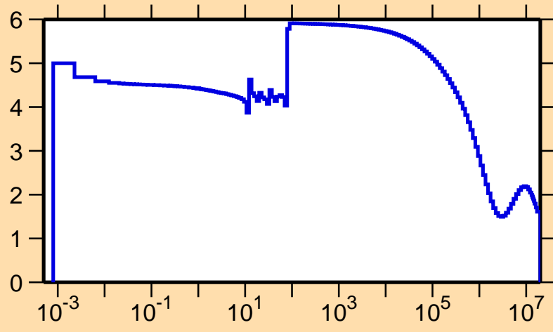
\sigma vs. E for ^{79}\text{Sr}(n,\text{el.})
