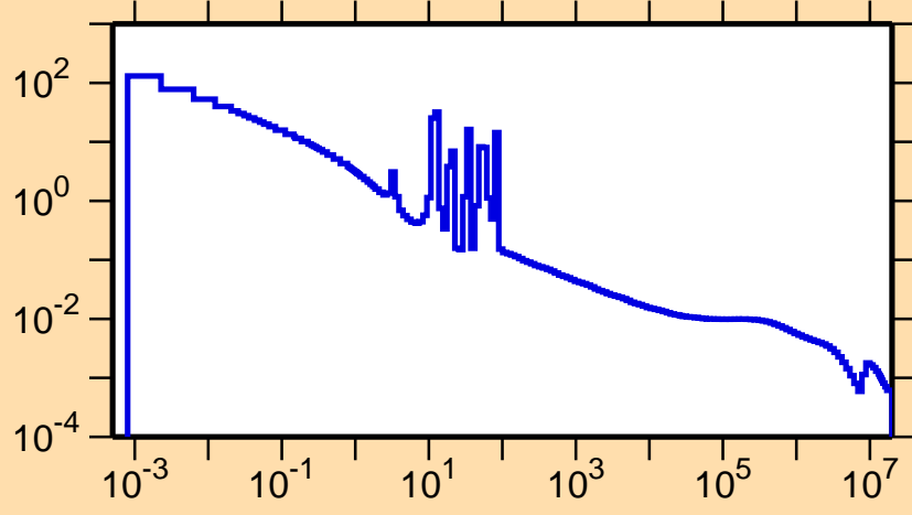
\sigma vs. E for ^{79}\text{Sr}(n,\gamma)
