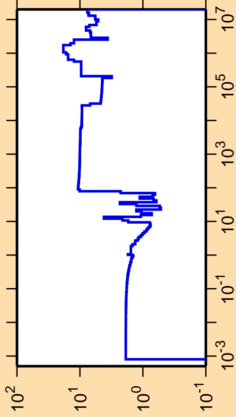
\Delta\sigma/\sigma vs. E for ^{79}\text{Sr}(n,\text{el.})
