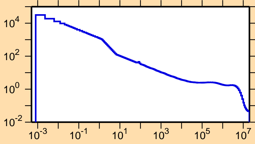
\sigma vs. E for ^{79}\text{Sr}(n,p)
