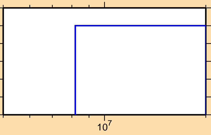
\sigma vs. E for ^{79}\text{Sr}(n,2n)
