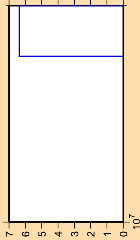
\Delta\sigma/\sigma vs. E for ^{80}\text{Sr}(n,2np)
