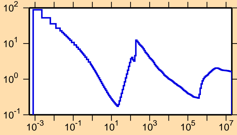
\sigma vs. E for ^{80}\text{Sr}(n,\text{nonel.})
