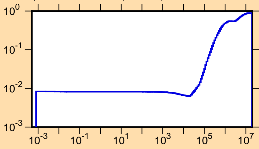
\mu vs. E for ^{81}\text{Sr}(\text{mt251})
