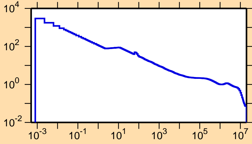
\sigma vs. E for ^{81}\text{Sr}(n,p)
