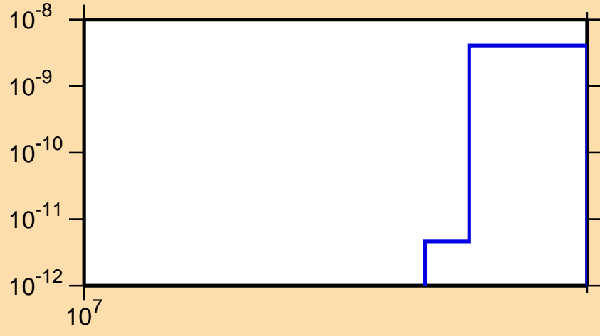
\sigma vs. E for ^{81}\text{Sr} (mt 34)
