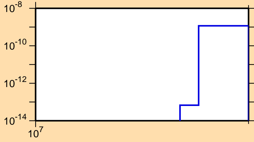
\sigma vs. E for ^{81}\text{Sr} (mt 45)
