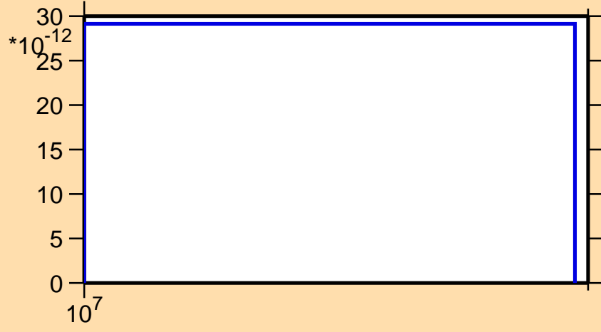
\sigma vs. E for ^{81}\text{Sr} (mt 34)
