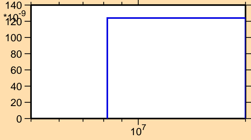
\sigma vs. E for ^{81}\text{Sr}(n,\text{nd})
