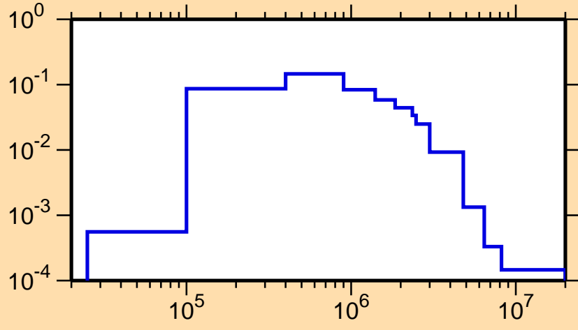
\sigma vs. E for ^{81}\text{Sr}(n,n_1)
