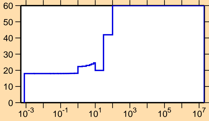
\Delta\sigma/\sigma vs. E for ^{81}\text{Sr}(n,\gamma)
