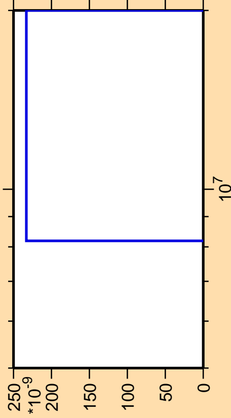
\Delta\sigma/\sigma vs. E for ^{81}\text{Sr}(n,nt)
