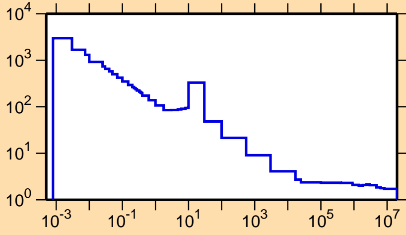
\sigma vs. E for ^{81}\text{Sr}(n,\text{nonel.})
