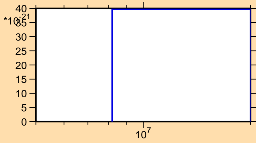
\sigma vs. E for ^{81}\text{Sr}(n,nt)
