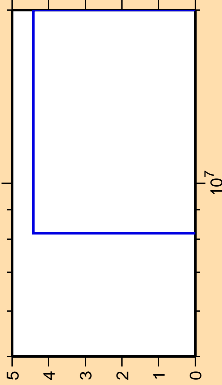
\Delta\sigma/\sigma vs. E for ^{81}\text{Sr}(\text{mt117})
