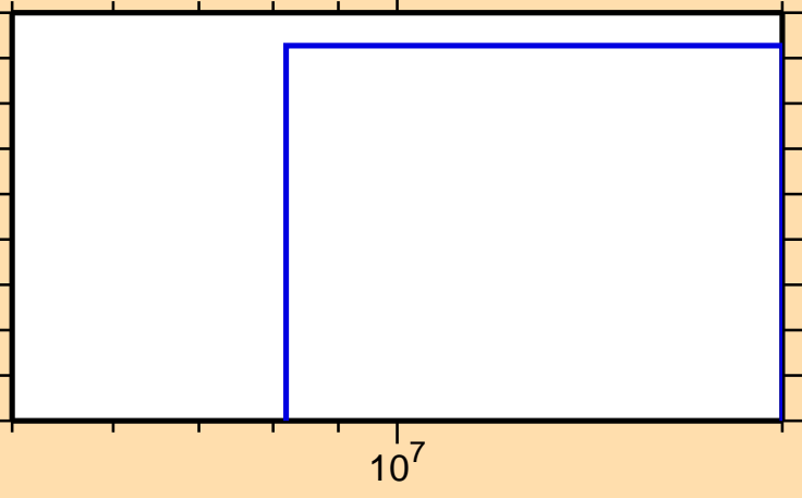
\sigma vs. E for ^{83}\text{Sr}(n,\text{pd})
