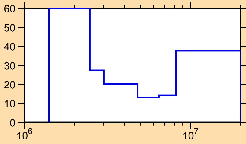
\Delta\sigma/\sigma vs. E for ^{83}\text{Sr}(n,ncont.)
