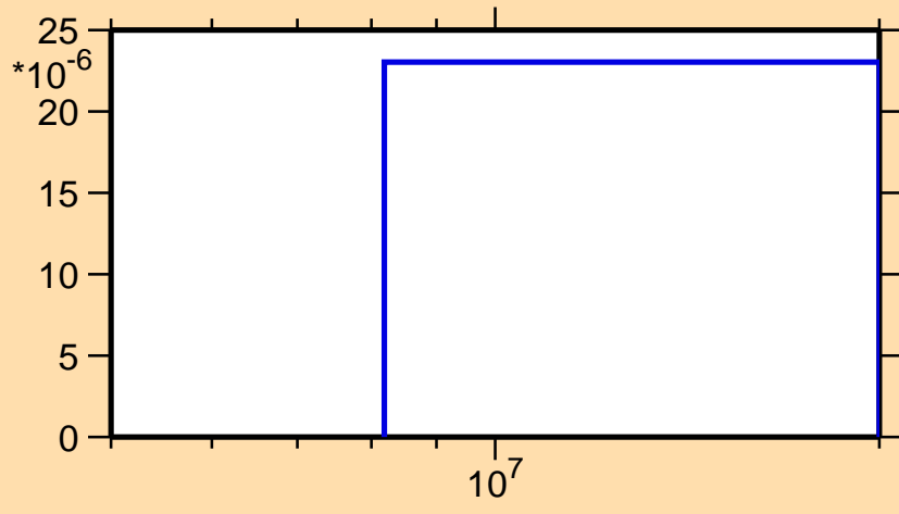
\sigma vs. E for ^{83}\text{Sr}(n,t)
