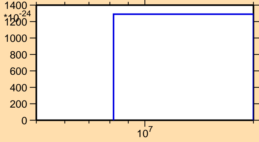
\sigma vs. E for ^{83}\text{Sr}(n,nt)
