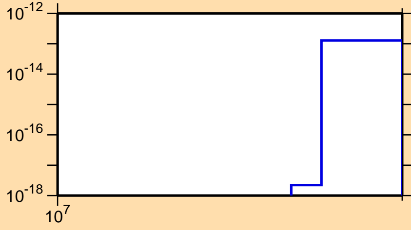
\sigma vs. E for ^{83}\text{Sr}(\text{mt117})
