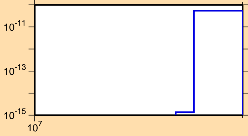
\sigma vs. E for ^{83}\text{Sr} (mt 34)
