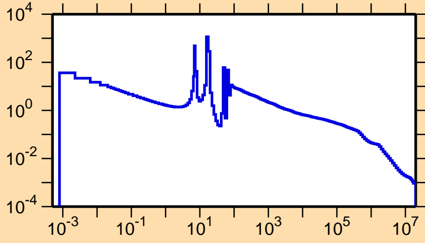
\sigma vs. E for ^{83}\text{Sr}(n,\gamma)
