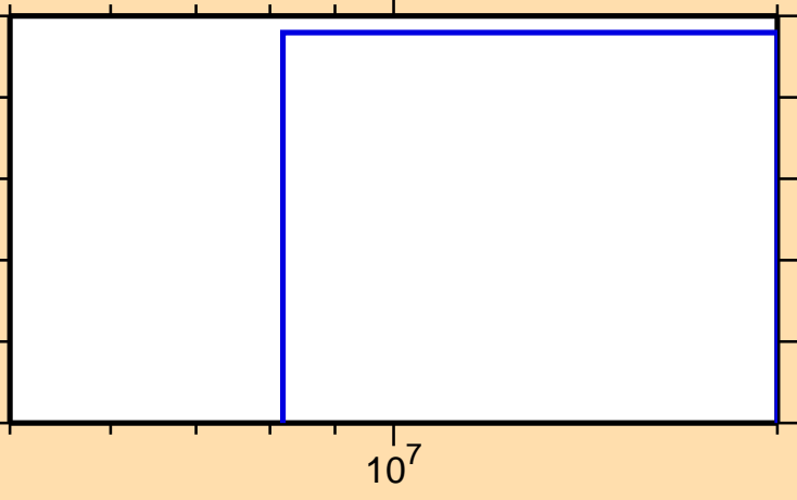
\sigma vs. E for ^{83}\text{Sr}(n,\text{pd})
