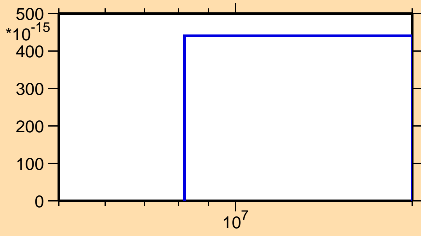
\sigma vs. E for ^{83}\text{Sr}(\text{mt } 34)
