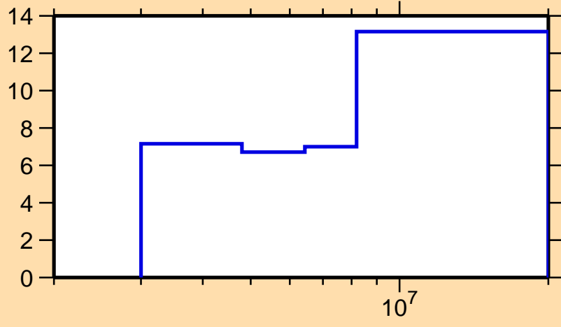
\Delta\sigma/\sigma vs. E for ^{84}\text{Sr}(n,inel.)
