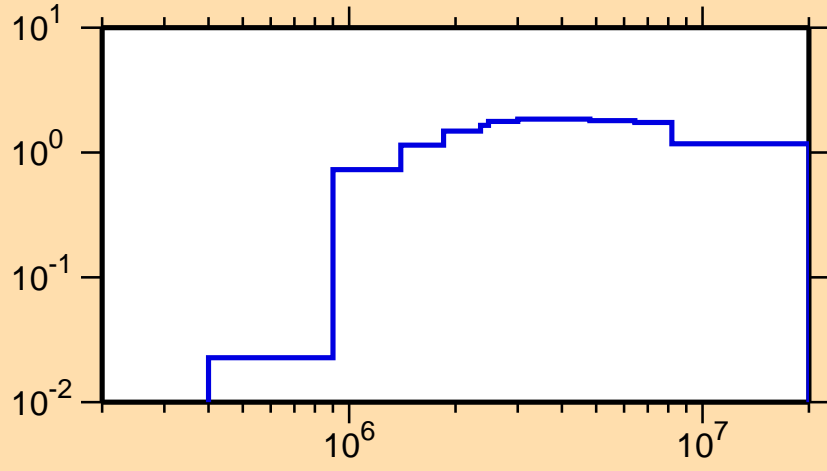
\sigma vs. E for ^{84}\text{Sr}(n,\text{inel.})
