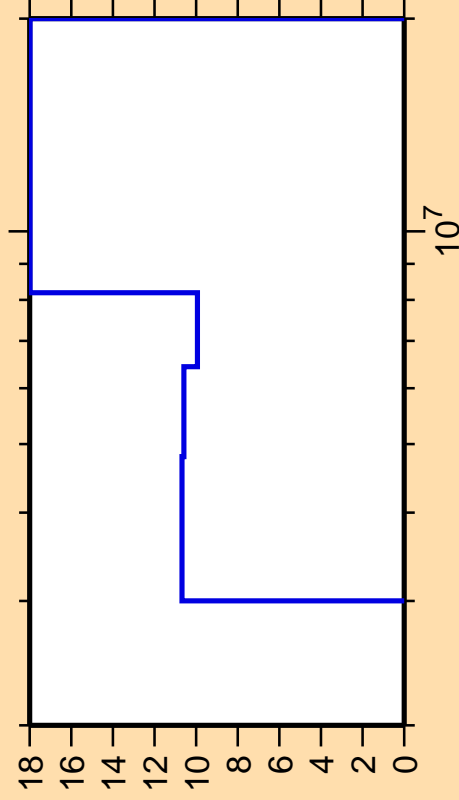
\Delta\sigma/\sigma vs. E for ^{84}\text{Sr}(n,ncont.)
