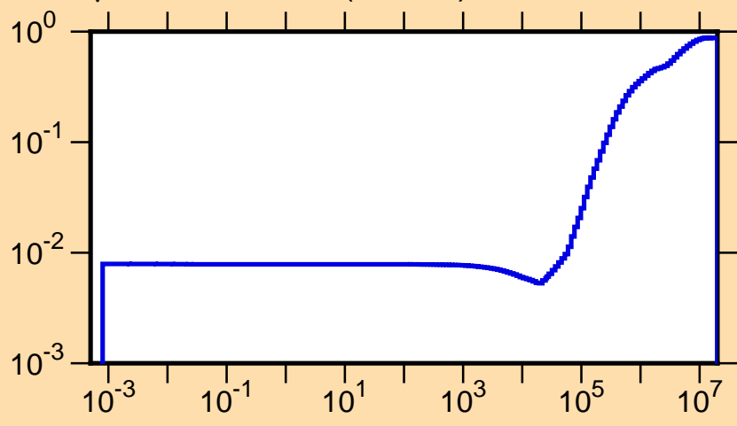
\mu vs. E for ^{85}\text{Sr}(\text{mt251})
