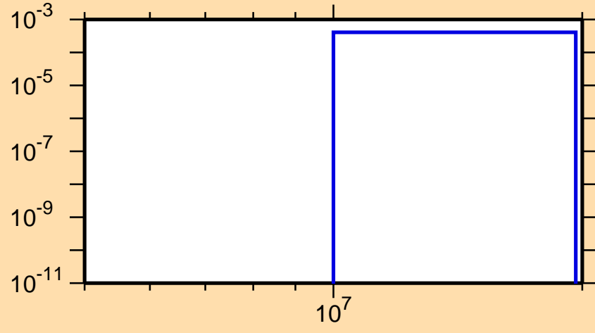
\sigma vs. E for ^{85}\text{Sr}(n,\alpha)
