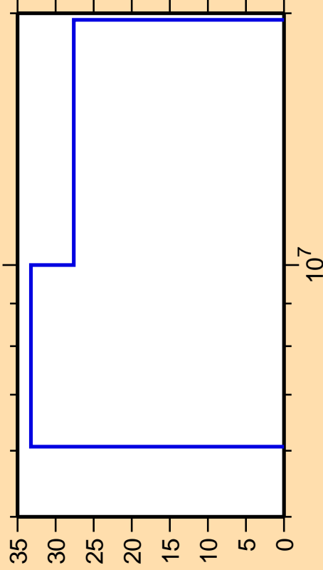
\Delta\sigma/\sigma vs. E for ^{85}\text{Sr}(n,2n)
