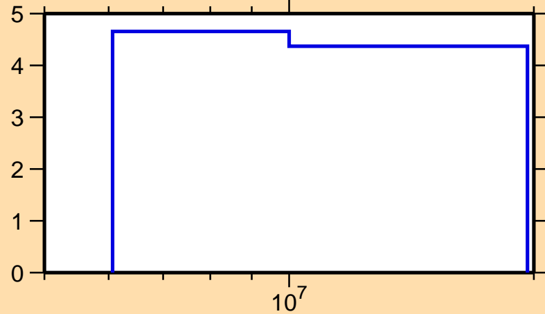
\Delta\sigma/\sigma vs. E for ^{85}\text{Sr}(n,\text{nonel.})
