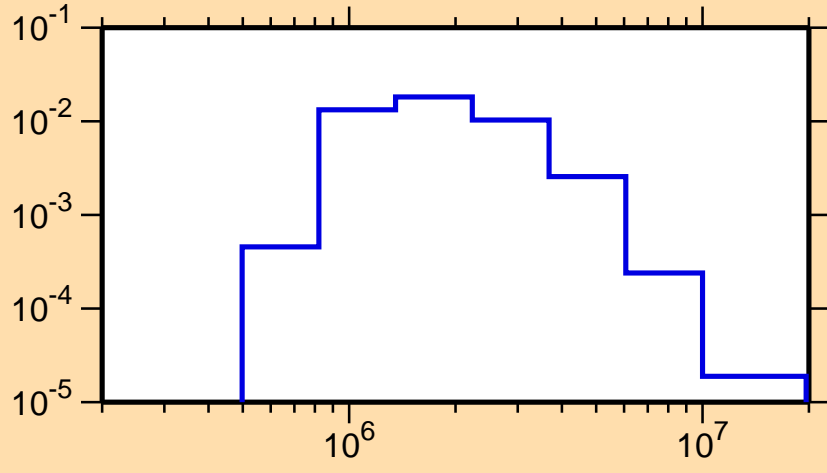
\sigma vs. E for ^{85}\text{Sr}(n,n_3)
