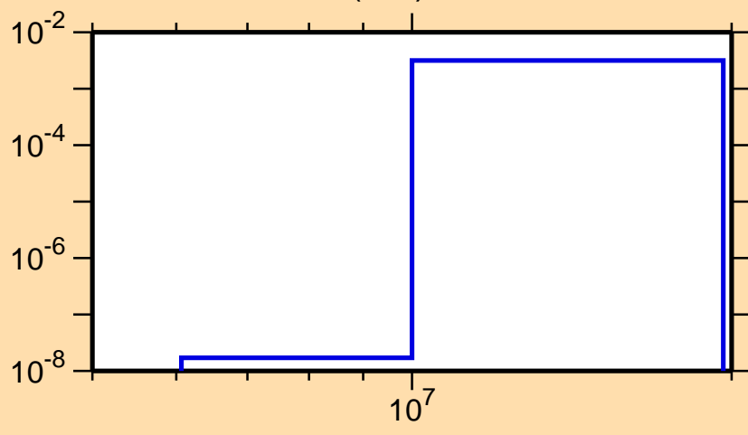
\sigma vs. E for ^{85}\text{Sr}(n,d)
