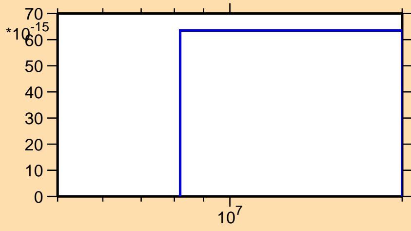
\sigma vs. E for ^{85}\text{Sr}(n,\text{pt})
