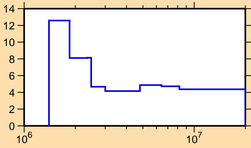
\Delta\sigma/\sigma vs. E for ^{85}\text{Sr}(n,\text{nonel.})
