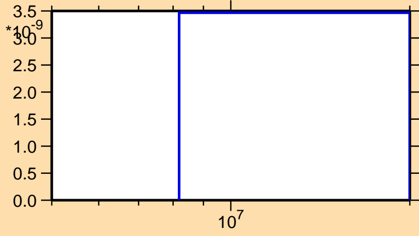
\sigma vs. E for ^{85}\text{Sr}(n,2np)
