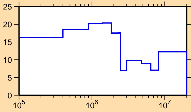
\Delta\sigma/\sigma vs. E for ^{85}\text{Sr}(n,\text{el.})
