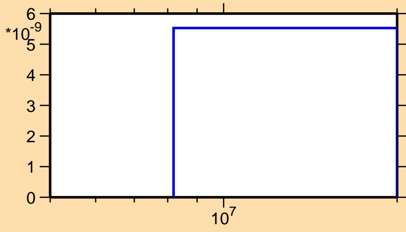
\sigma vs. E for ^{85}\text{Sr}(n,\text{nd})
