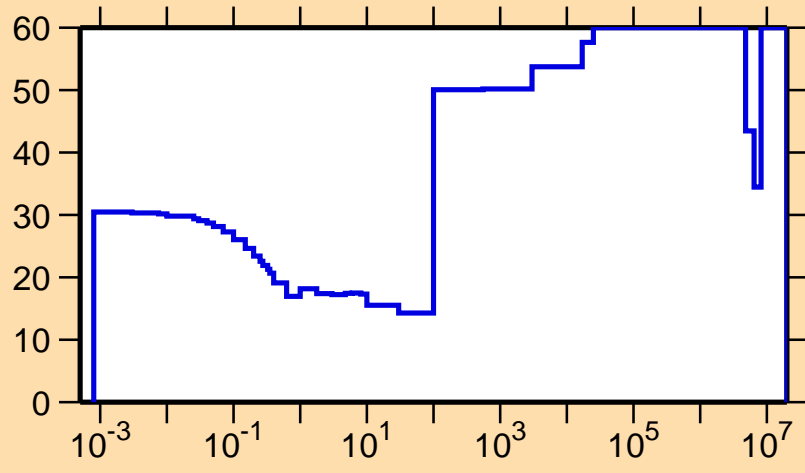
\Delta\sigma/\sigma vs. E for ^{85}\text{Sr}(n,\gamma)
