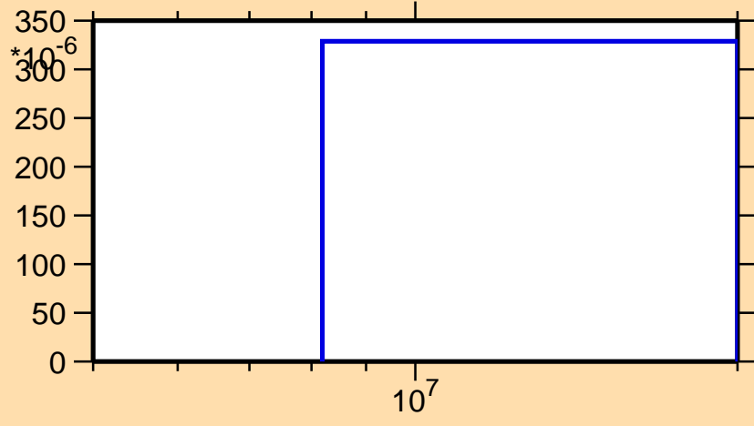
\sigma vs. E for ^{85}\text{Sr}(n,n\alpha)
