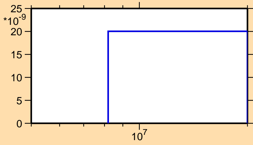
\sigma vs. E for ^{85}\text{Sr}(n,p\alpha)
