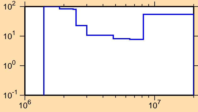
\Delta\sigma/\sigma vs. E for ^{85}\text{Sr}(n,n\text{cont.})
