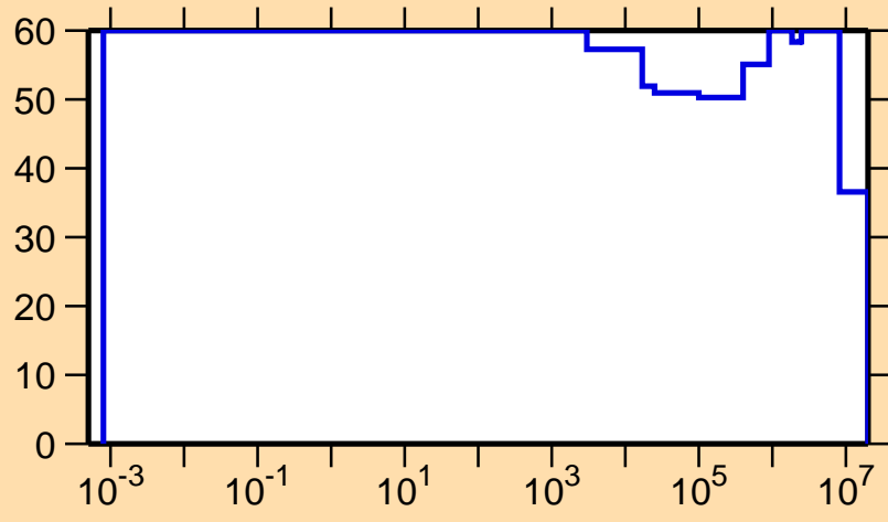
\Delta\sigma/\sigma vs. E for ^{85}\text{Sr}(n,p)
