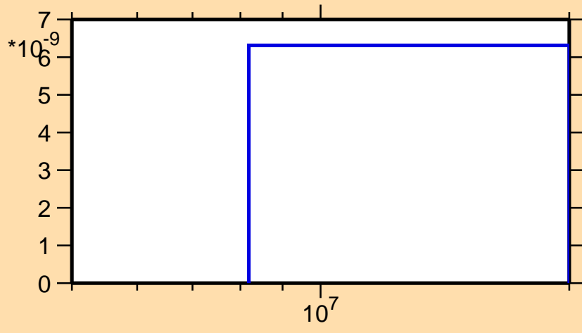
\sigma vs. E for ^{85}\text{Sr}(n,\text{He3})
