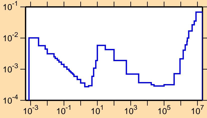
\sigma vs. E for ^{85}\text{Sr}(n,p)
