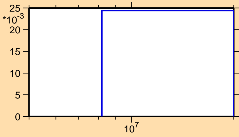
\sigma vs. E for ^{85}\text{Sr}(n,np)
