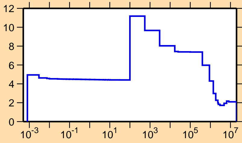
\sigma vs. E for ^{85}\text{Sr}(n,\text{el.})
