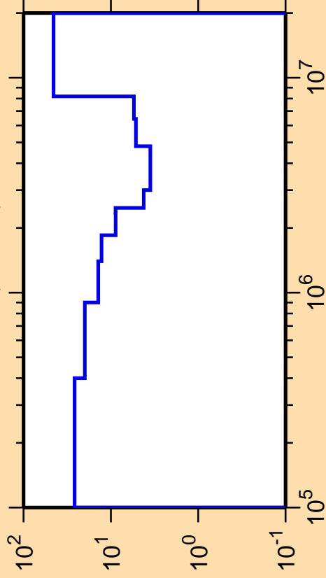
\Delta\sigma/\sigma vs. E for ^{85}\text{Sr}(n,\text{inel.})
