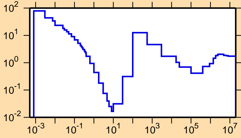
\sigma vs. E for ^{85}\text{Sr}(n,\text{nonel.})
