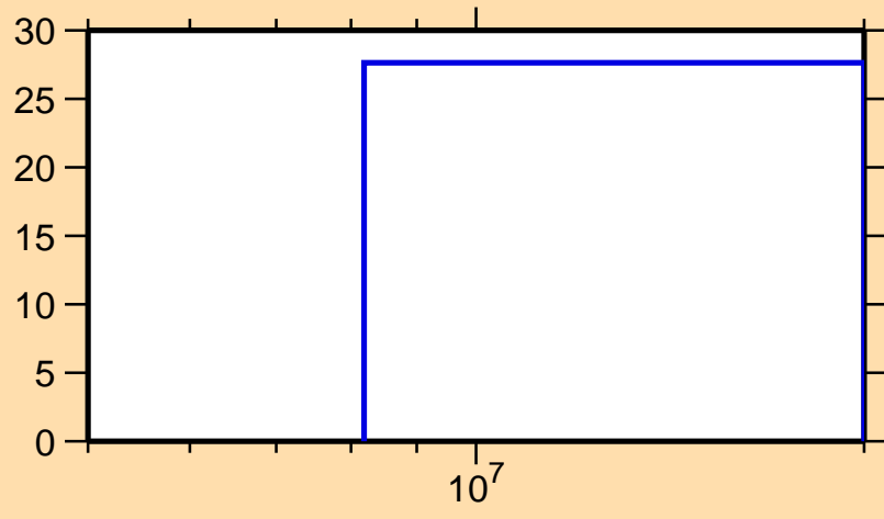
\Delta\sigma/\sigma vs. E for ^{85}\text{Sr}(n,2n)
