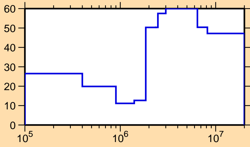
\Delta\sigma/\sigma vs. E for ^{85}\text{Sr}(n,n_1)
