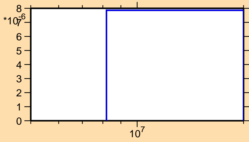
\sigma vs. E for ^{85}\text{Sr}(n,t)
