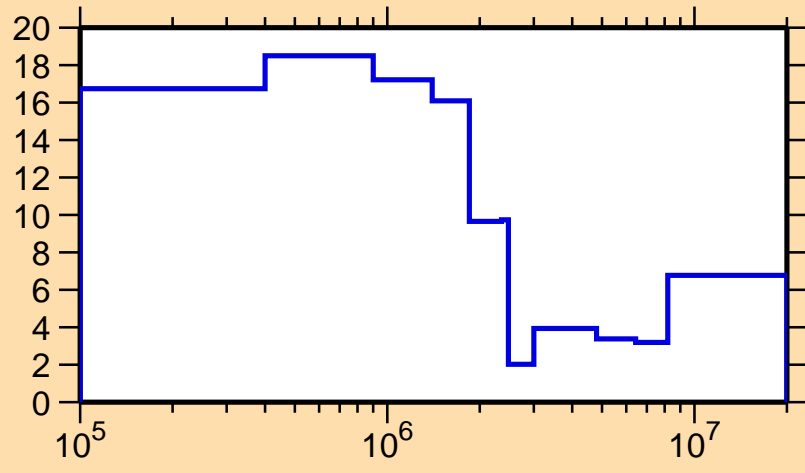
\Delta\sigma/\sigma vs. E for ^{85}\text{Sr}(n,\text{tot.})
