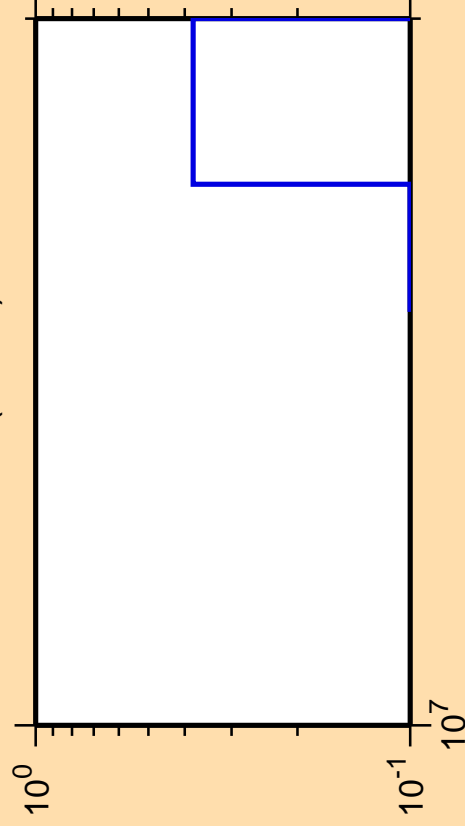
\Delta\sigma/\sigma vs. E for ^{85}\text{Sr} (mt 34)
