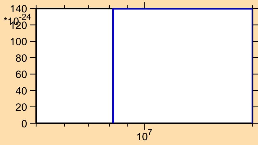
\sigma vs. E for ^{85}\text{Sr}(n,nt)
