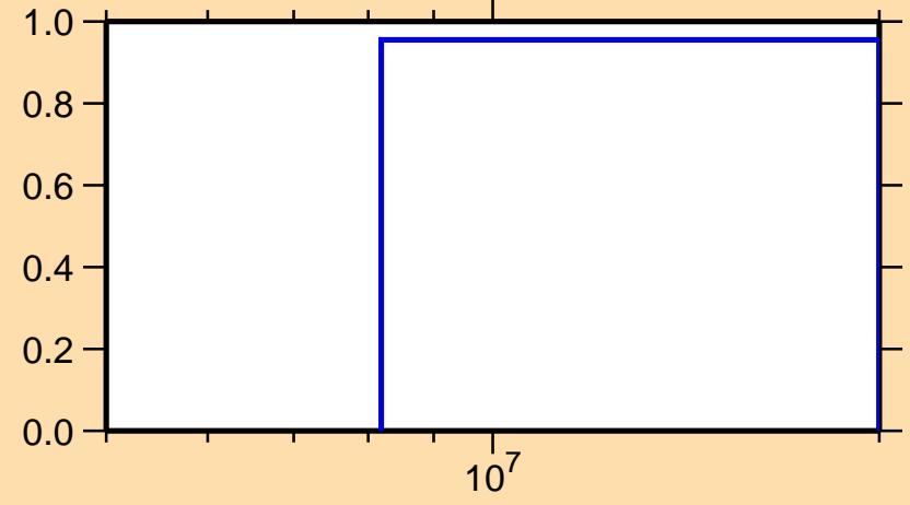
\sigma vs. E for ^{85}\text{Sr}(n,2n)
