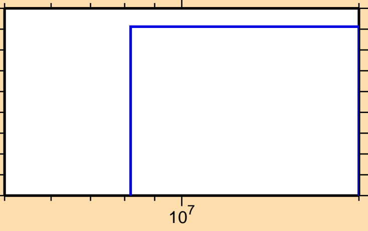
\sigma vs. E for ^{85}\text{Sr}(n,\text{nd})
