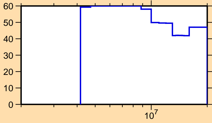
\Delta\sigma/\sigma vs. E for ^{88}\text{Sr}(n,\gamma)
