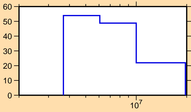
\Delta\sigma/\sigma vs. E for ^{88}\text{Sr}(n,p)
