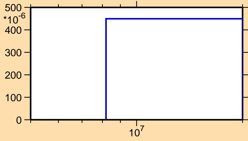
\sigma vs. E for ^{88}\text{Sr}(n,d)
