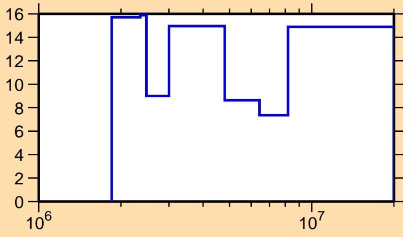
\Delta\sigma/\sigma vs. E for ^{88}\text{Sr}(n,\text{el.})
