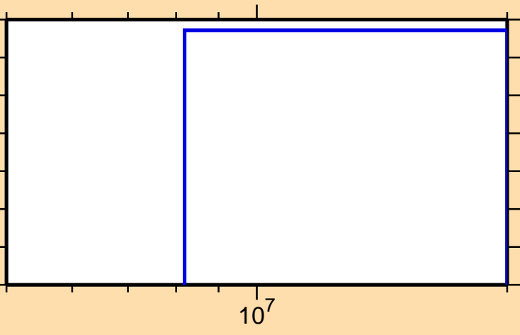
\sigma vs. E for ^{88}\text{Sr}(n,t)
