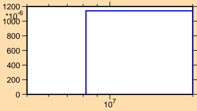
\sigma vs. E for ^{88}\text{Sr}(n,np)
