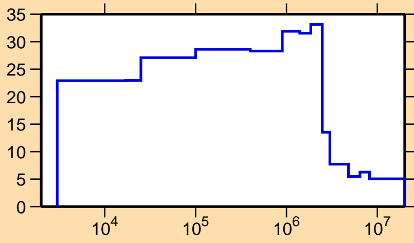
\Delta\sigma/\sigma vs. E for ^{88}\text{Sr}(n,\text{nonel.})
