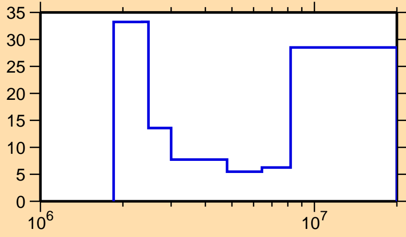
\Delta\sigma/\sigma vs. E for ^{88}\text{Sr}(n,\text{inel.})
