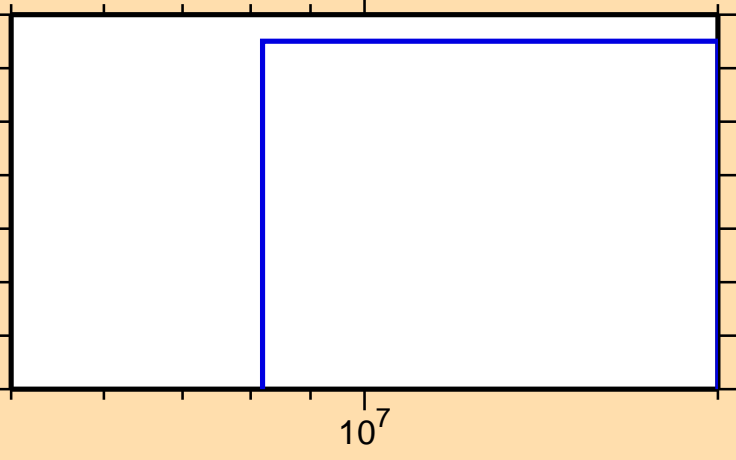
\sigma vs. E for ^{88}\text{Sr}(n,2n)
