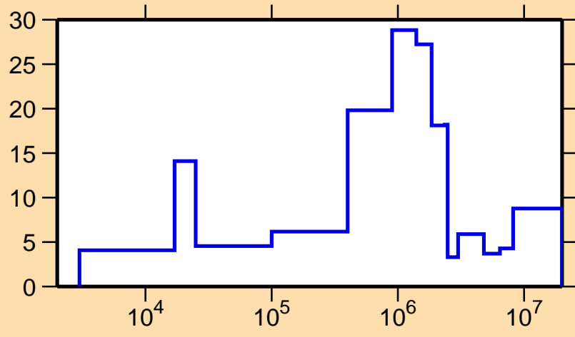
\Delta\sigma/\sigma vs. E for ^{88}\text{Sr}(n,\text{tot.})
