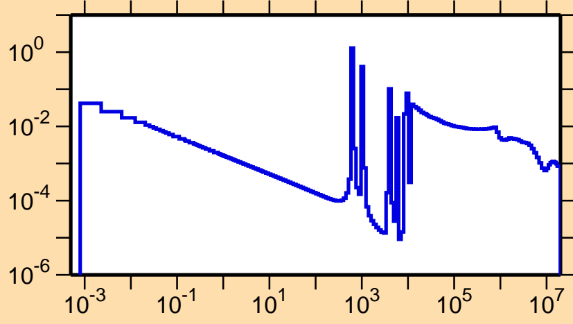
\sigma vs. E for ^{90}\text{Sr}(n,\gamma)
