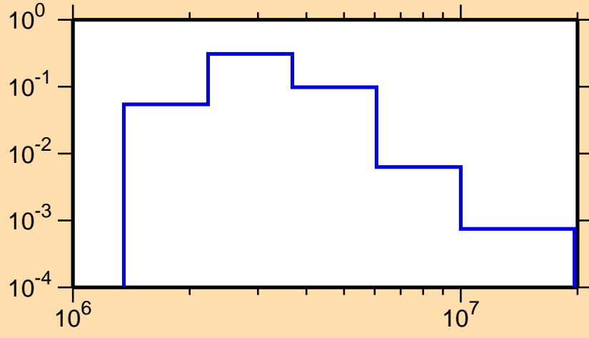
\sigma vs. E for ^{90}\text{Sr}(n,n_3)
