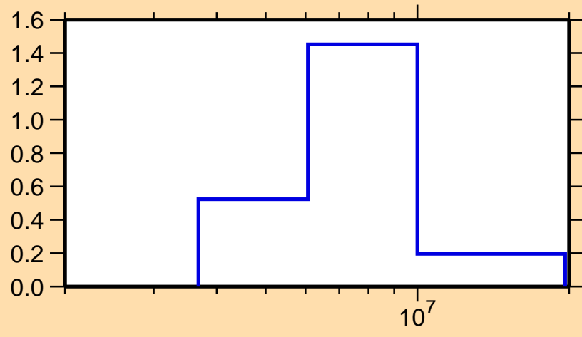
\sigma vs. E for ^{90}\text{Sr}(n,n\text{cont.})
