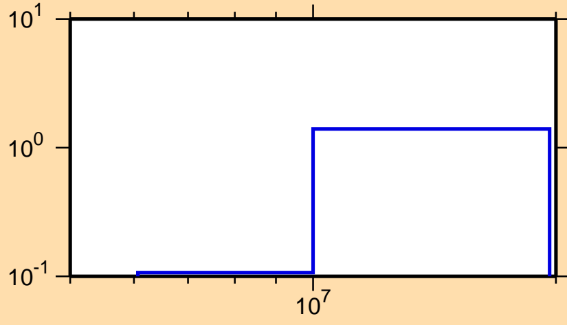
\sigma vs. E for ^{90}\text{Sr}(n,2n)
