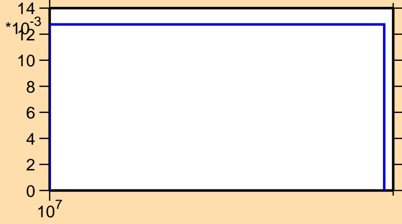
\sigma vs. E for ^{90}\text{Sr}(n,3n)
