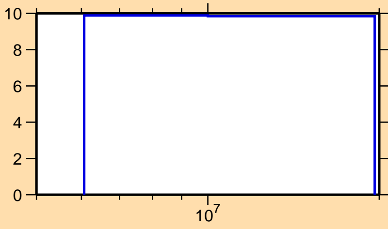
\Delta\sigma/\sigma vs. E for ^{90}\text{Sr}(n,2n)
