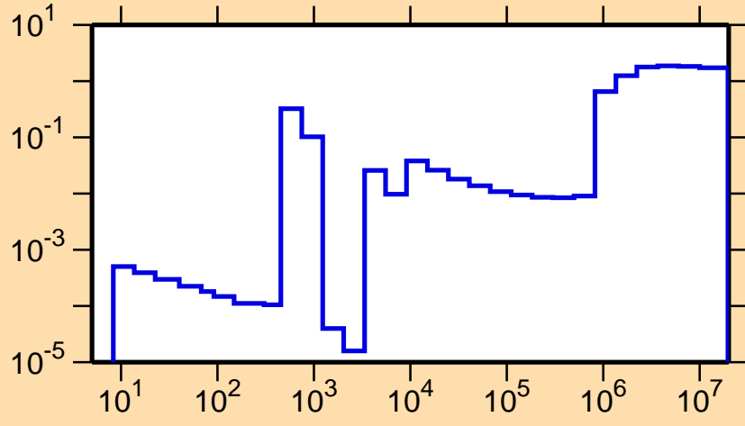
\sigma vs. E for ^{90}\text{Sr}(n,\text{nonel.})
