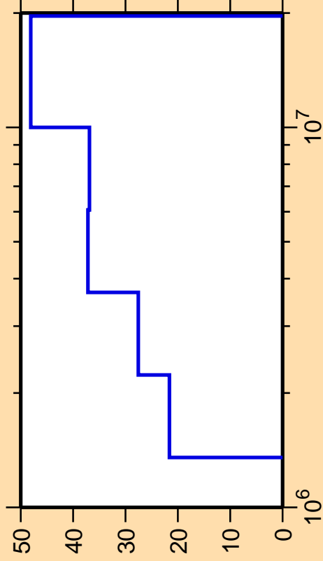
\Delta\sigma/\sigma vs. E for ^{90}\text{Sr}(n,n_3)
