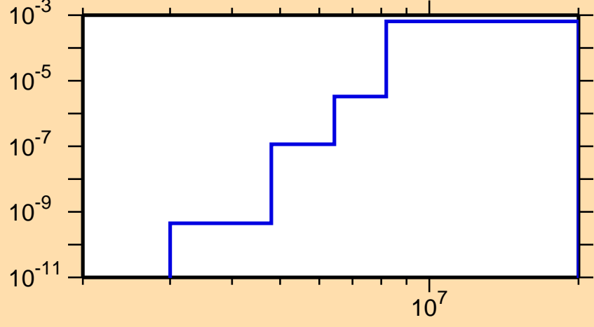
\sigma vs. E for ^{90}\text{Sr}(n,\alpha)
