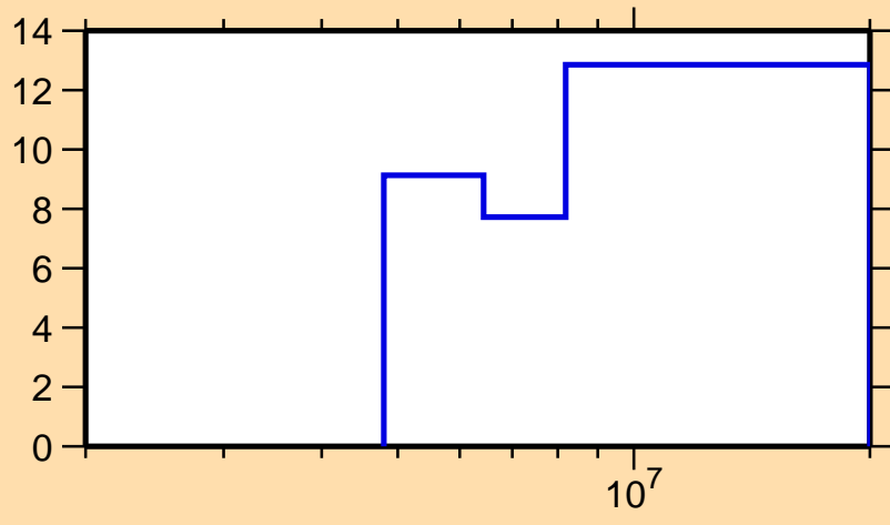
\Delta\sigma/\sigma vs. E for ^{90}\text{Sr}(n,el.)
