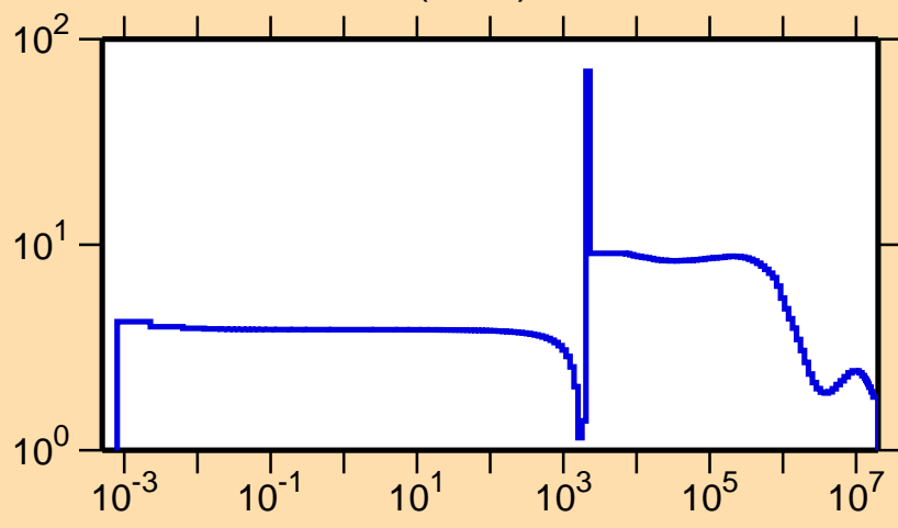
\sigma vs. E for ^{92}\text{Sr}(n,\text{el.})
