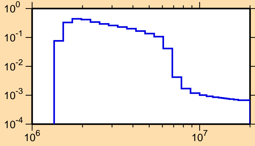
\sigma vs. E for ^{92}\text{Sr}(n,n_2)
