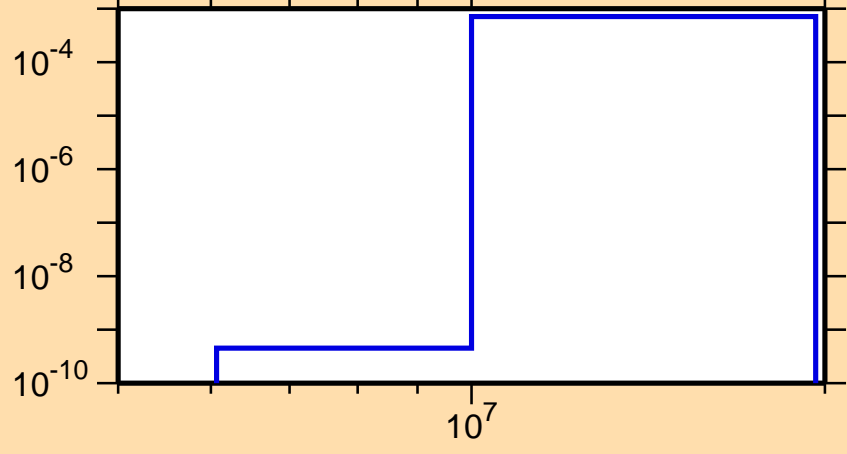
\sigma vs. E for ^{92}\text{Sr}(n,p)
