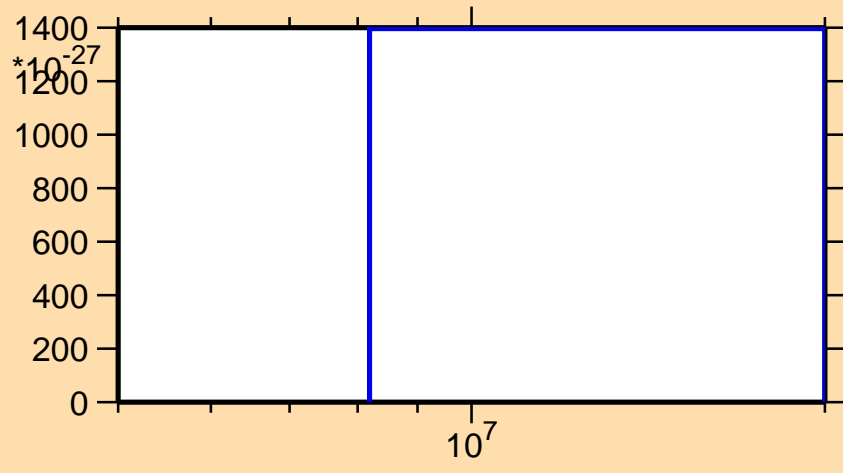
\sigma vs. E for ^{92}\text{Sr}(n,3n\alpha)
