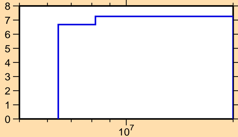
\Delta\sigma/\sigma vs. E for ^{92}\text{Sr}(n,\text{nonel.})
