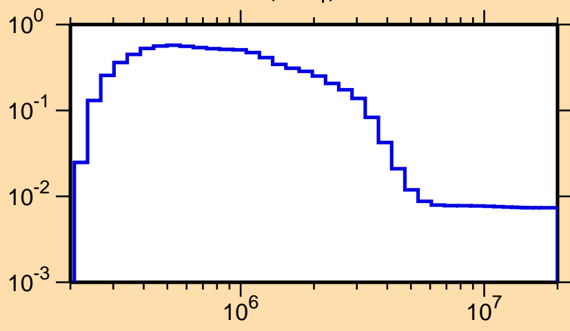
\sigma vs. E for ^{93}\text{Sr}(n,n_1)
