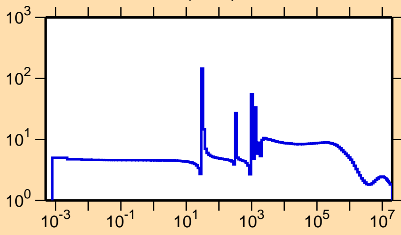
\sigma vs. E for ^{93}\text{Sr}(n,\text{el.})
