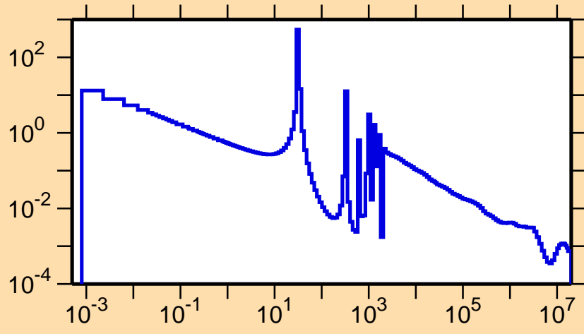
\sigma vs. E for ^{93}\text{Sr}(n,\gamma)
