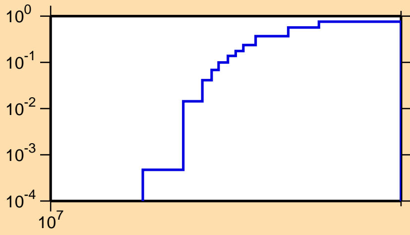
\sigma vs. E for ^{93}\text{Sr}(n,3n)
