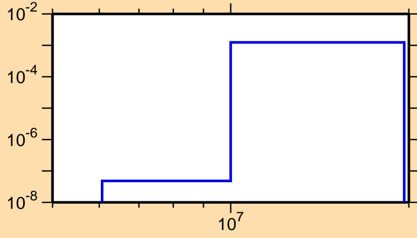
\sigma vs. E for ^{93}\text{Sr}(n,p)
