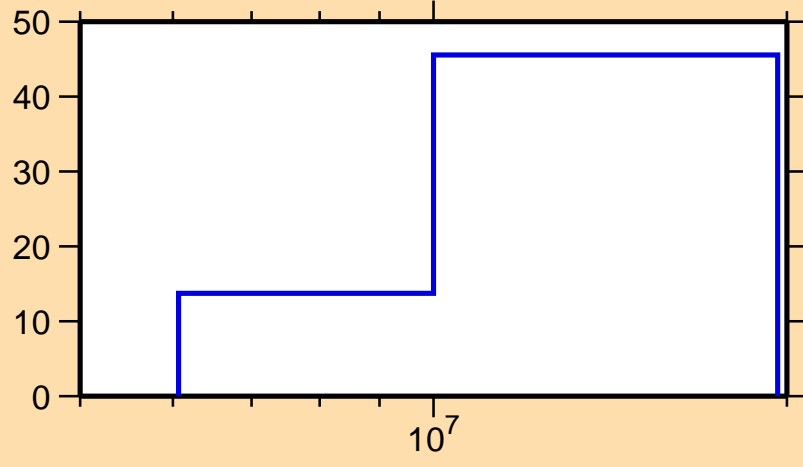
\Delta\sigma/\sigma vs. E for ^{93}\text{Sr}(n,ncont.)
