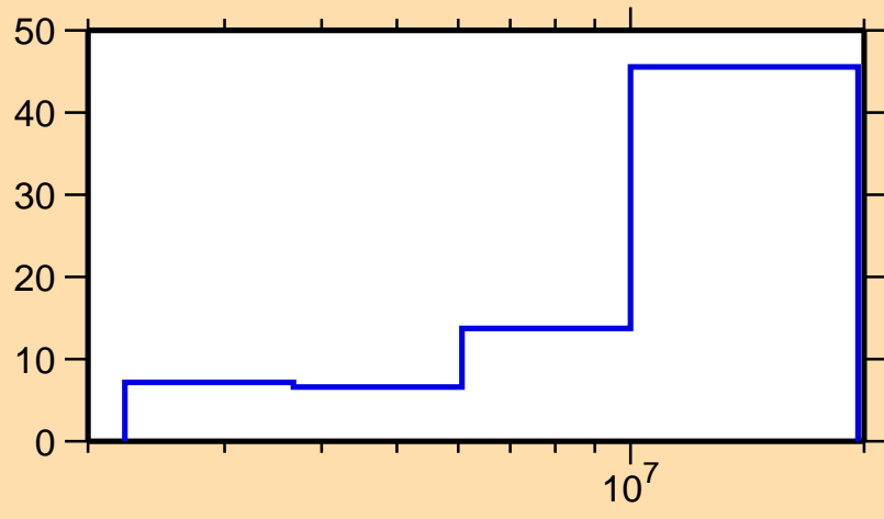
\Delta\sigma/\sigma vs. E for ^{93}\text{Sr}(n,n\text{cont.})
