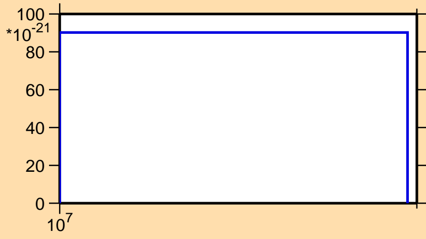
\sigma vs. E for ^{93}\text{Sr}(n,3n\alpha)
