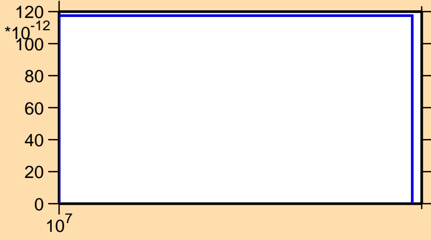
\sigma vs. E for ^{93}\text{Sr}(n,nt)
