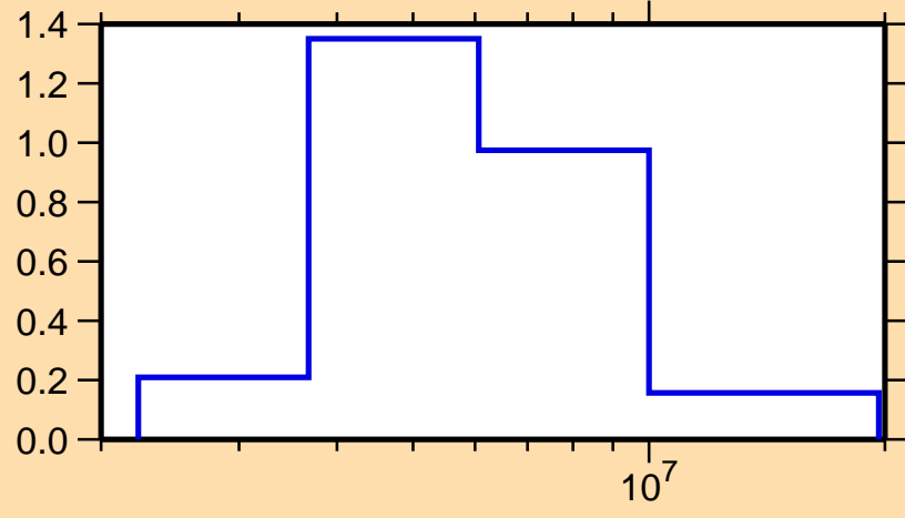
\sigma vs. E for ^{93}\text{Sr}(n,n\text{cont.})
