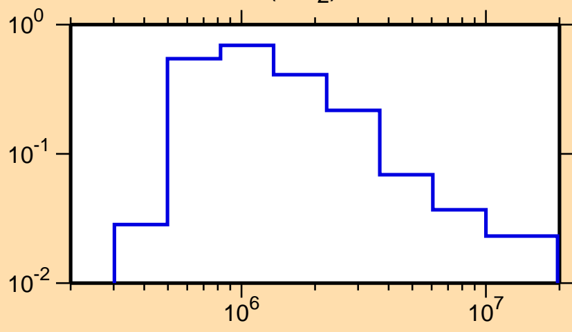
\sigma vs. E for ^{93}\text{Sr}(n,n_2)
