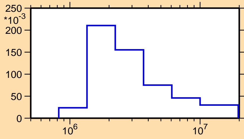
\sigma vs. E for ^{93}\text{Sr}(n,n_4)
