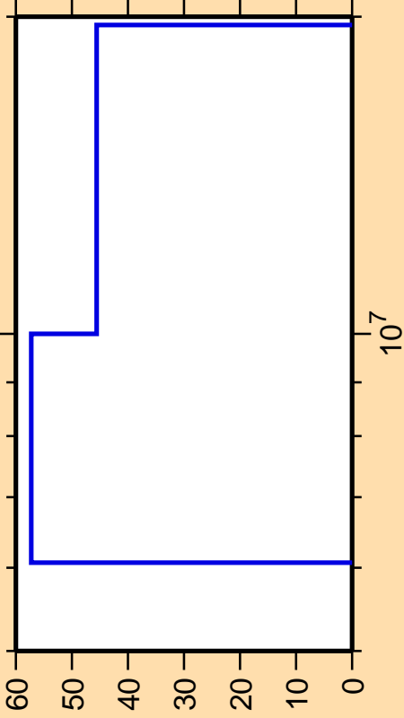
\Delta\sigma/\sigma vs. E for ^{93}\text{Sr}(n,p)
