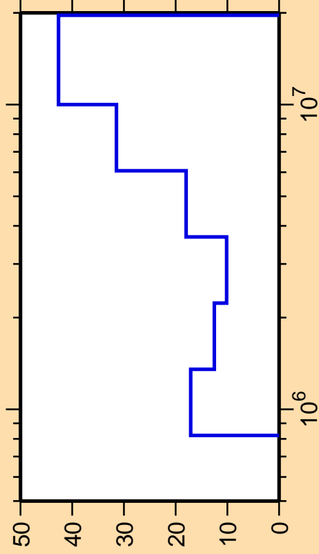
\Delta\sigma/\sigma vs. E for ^{93}\text{Sr}(n,n_4)
