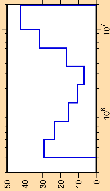
\Delta\sigma/\sigma vs. E for ^{93}\text{Sr}(n,n_2)
