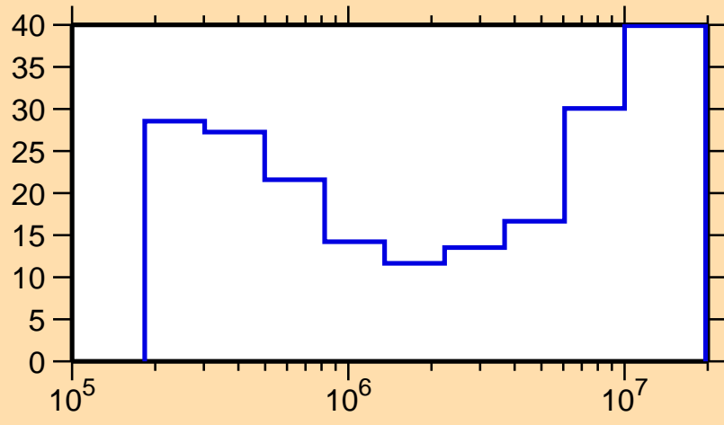
\Delta\sigma/\sigma vs. E for ^{93}\text{Sr}(n,n_1)
