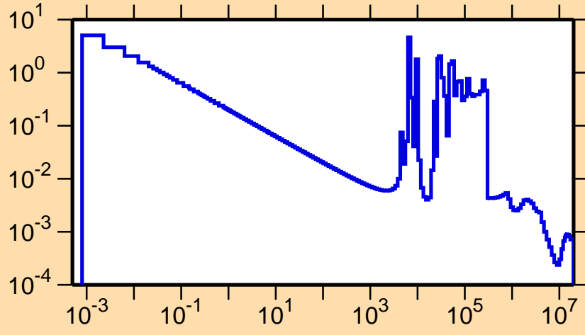
\sigma vs. E for ^{94}\text{Sr}(n,\gamma)
