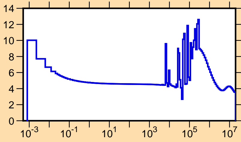
\sigma vs. E for ^{94}\text{Sr}(n,\text{tot.})
