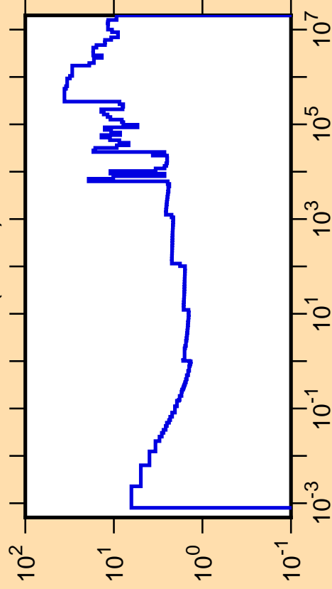
\Delta\sigma/\sigma vs. E for ^{94}\text{Sr}(n,\text{tot.})
