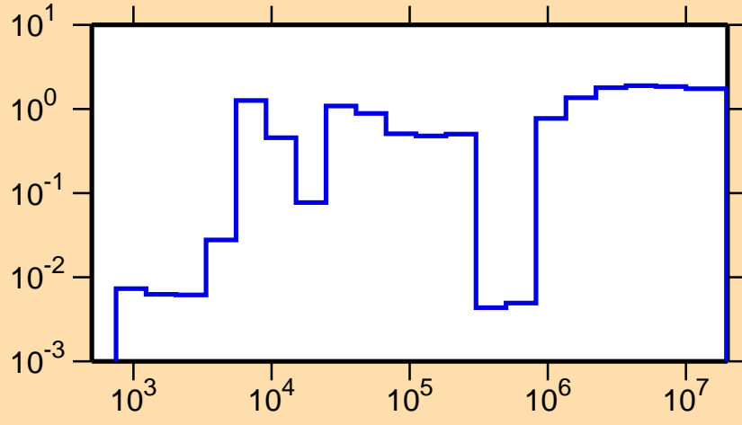
\sigma vs. E for ^{94}\text{Sr}(n,\text{nonel.})
