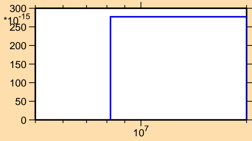
\sigma vs. E for ^{94}\text{Sr}(n,\text{nd})
