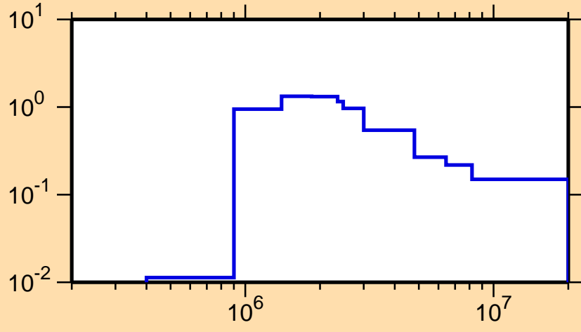
\sigma vs. E for ^{94}\text{Sr}(n,n_1)
