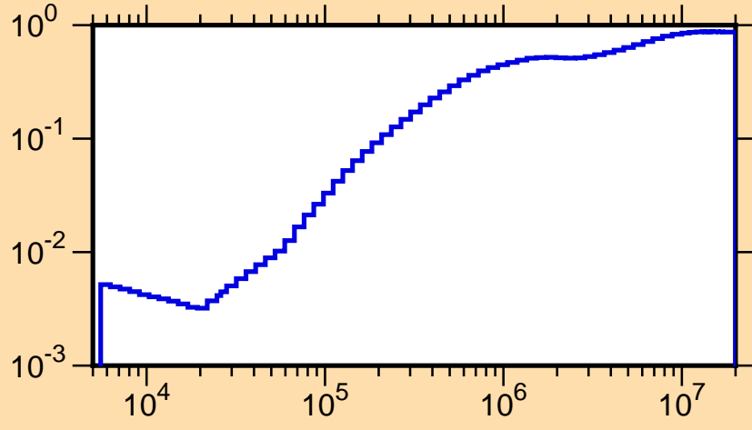
\mu vs. E for ^{95}\text{Sr}(\text{mt251})
